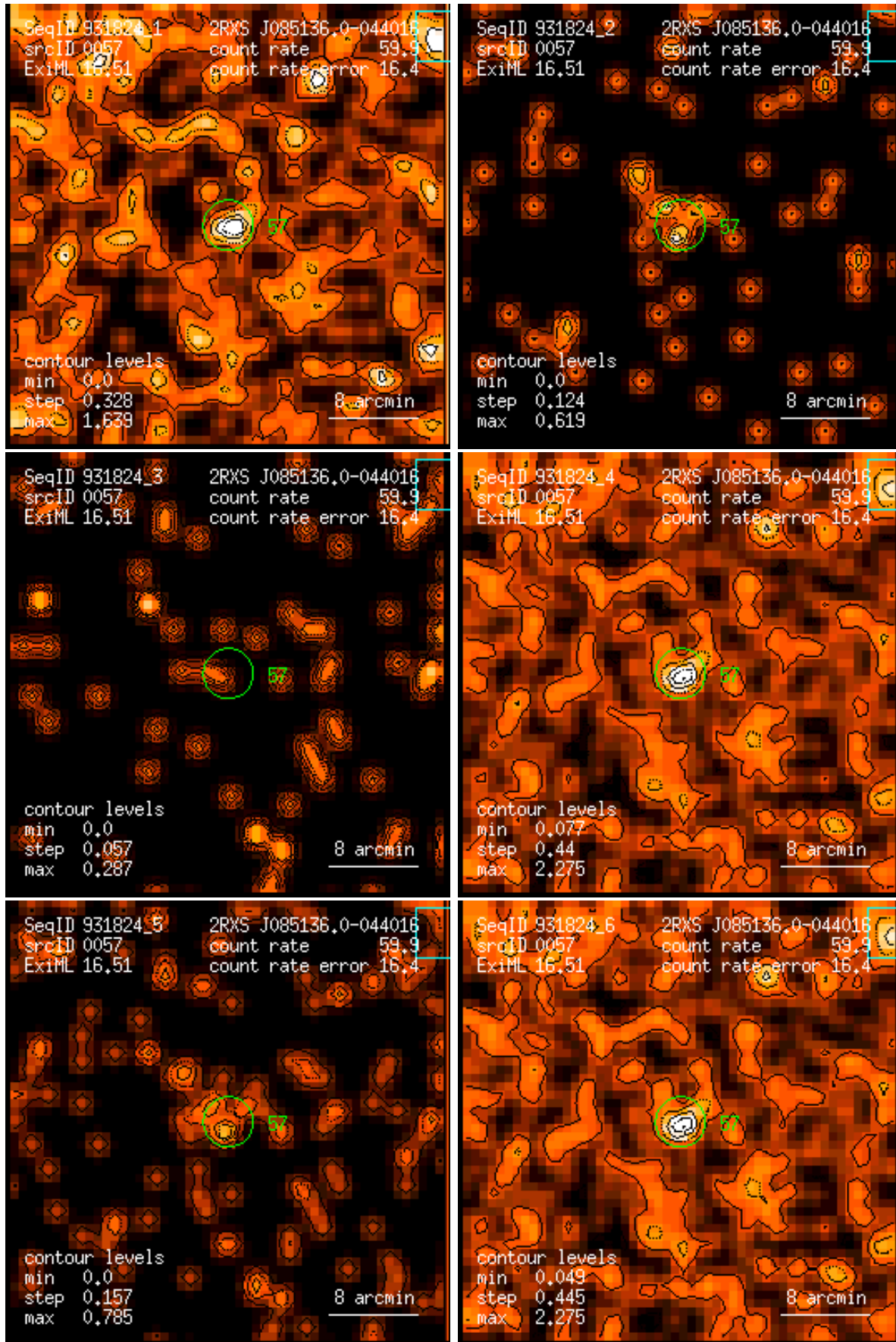
Figure 57: RASS 931824: detection 0057: band rate images, Gaussian filter: (1) PSPC channels 11 – 41, (2) 52 – 90, (3) 91 – 201, (4) 11 – 235, (5) 52 – 201, (6) 11 – 201. Broad band rates in counts/ks. Band rate contour levels in counts/ks/arcmin 2 .
