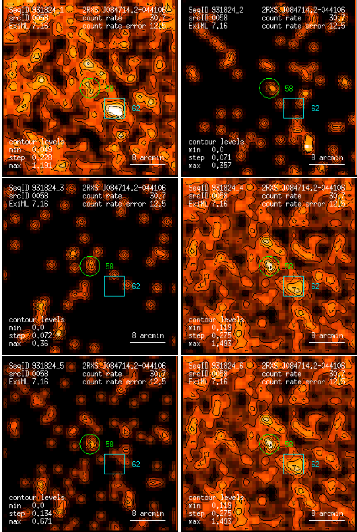
Figure 58: RASS 931824: detection 0058: band rate images, Gaussian filter: (1) PSPC channels 11 – 41, (2) 52 – 90, (3) 91 – 201, (4) 11 – 235, (5) 52 – 201, (6) 11 – 201. Broad band rates in counts/ks. Band rate contour levels in counts/ks/arcmin 2 .
