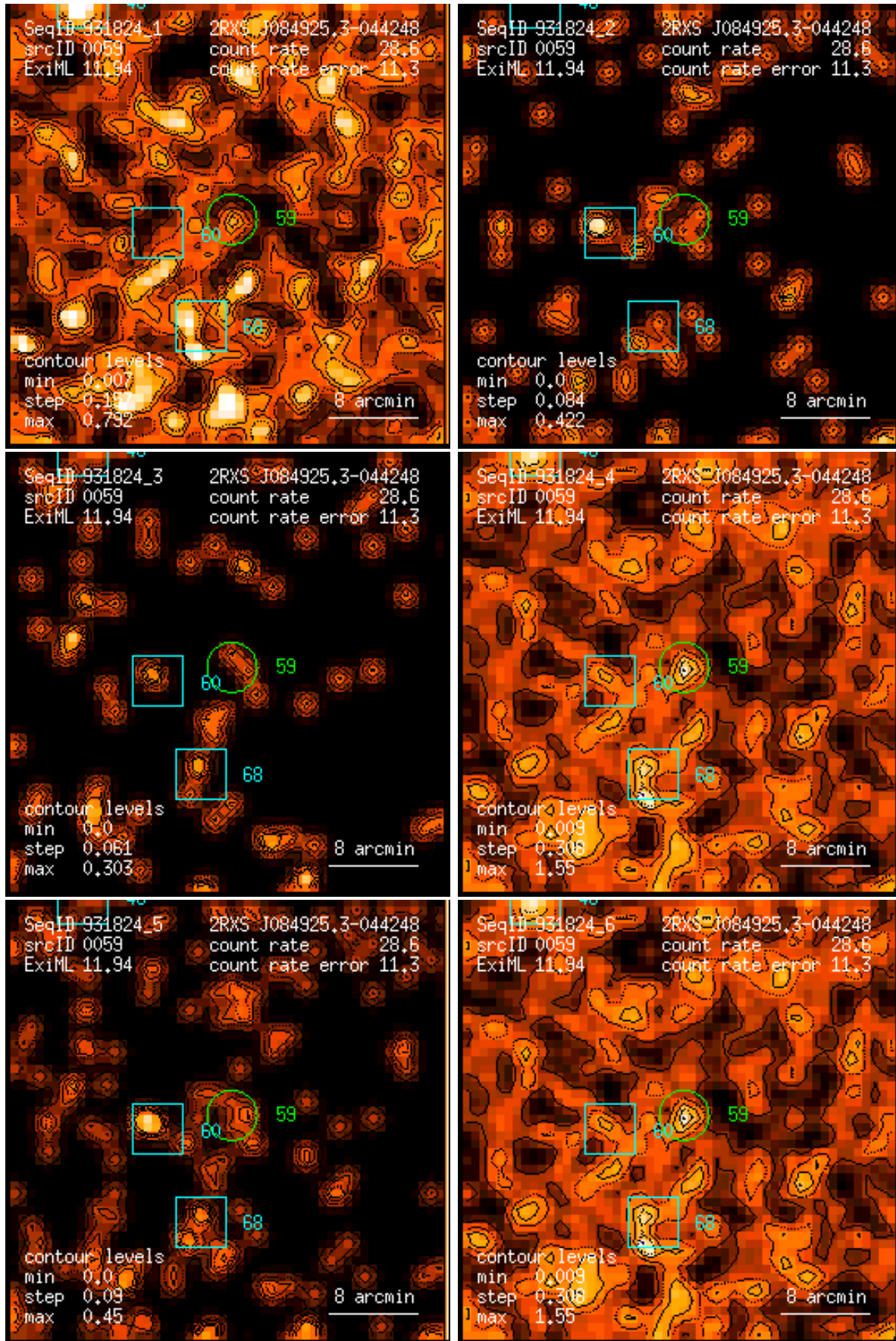
Figure 59: RASS 931824: detection 0059: band rate images, Gaussian filter: (1) PSPC channels 11 – 41, (2) 52 – 90, (3) 91 – 201, (4) 11 – 235, (5) 52 – 201, (6) 11 – 201. Broad band rates in counts/ks. Band rate contour levels in counts/ks/arcmin 2 .
