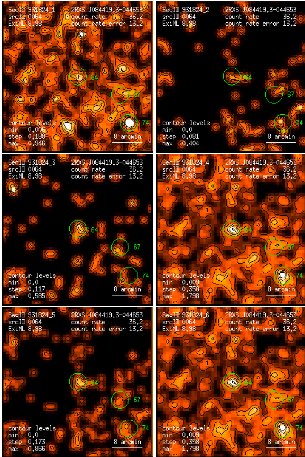
Figure 64: RASS 931824: detection 0064: band rate images, Gaussian filter: (1) PSPC channels 11 – 41, (2) 52 – 90, (3) 91 – 201, (4) 11 – 235, (5) 52 – 201, (6) 11 – 201. Broad band rates in counts/ks. Band rate contour levels in counts/ks/arcmin 2 .
