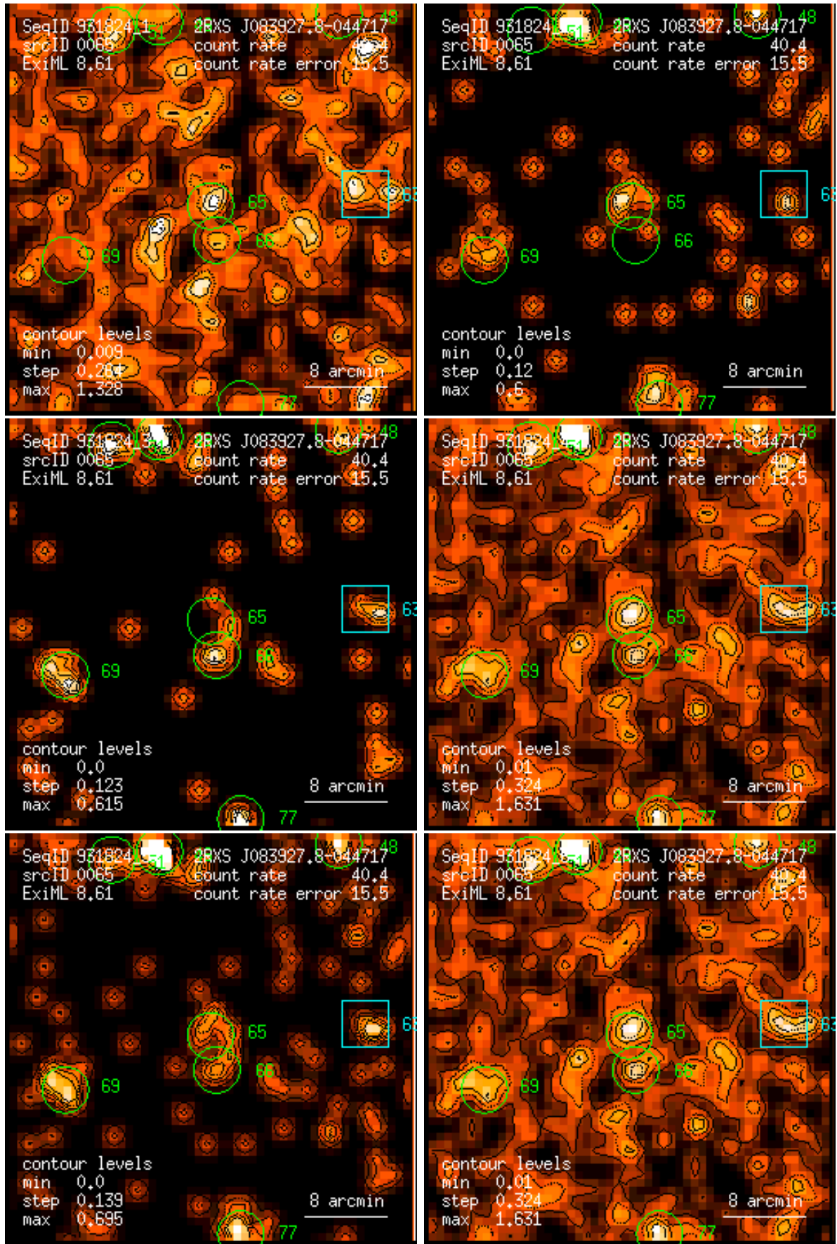
Figure 65: RASS 931824: detection 0065: band rate images, Gaussian filter: (1) PSPC channels 11 – 41, (2) 52 – 90, (3) 91 – 201, (4) 11 – 235, (5) 52 – 201, (6) 11 – 201. Broad band rates in counts/ks. Band rate contour levels in counts/ks/arcmin 2 .
