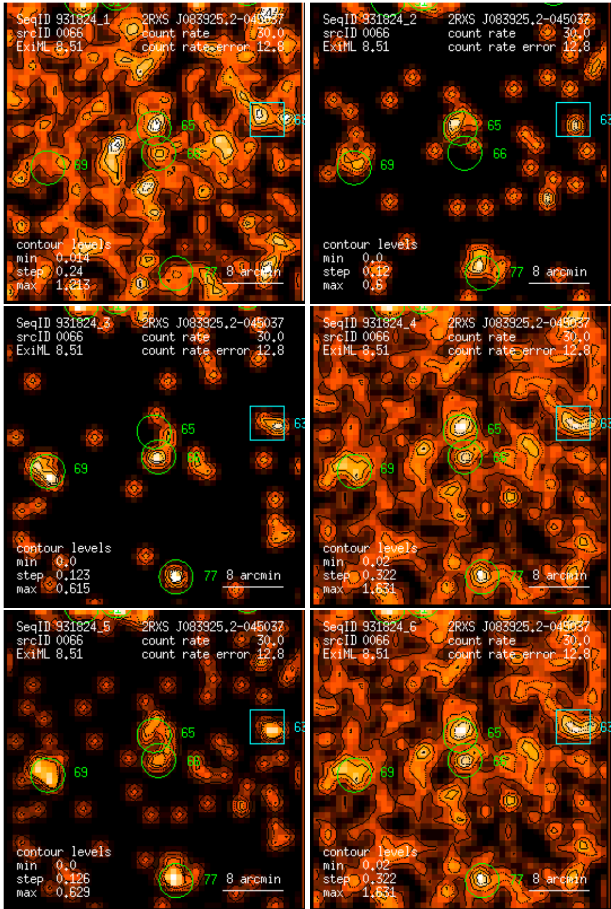
Figure 66: RASS 931824: detection 0066: band rate images, Gaussian filter: (1) PSPC channels 11 – 41, (2) 52 – 90, (3) 91 – 201, (4) 11 – 235, (5) 52 – 201, (6) 11 – 201. Broad band rates in counts/ks. Band rate contour levels in counts/ks/arcmin 2 .
