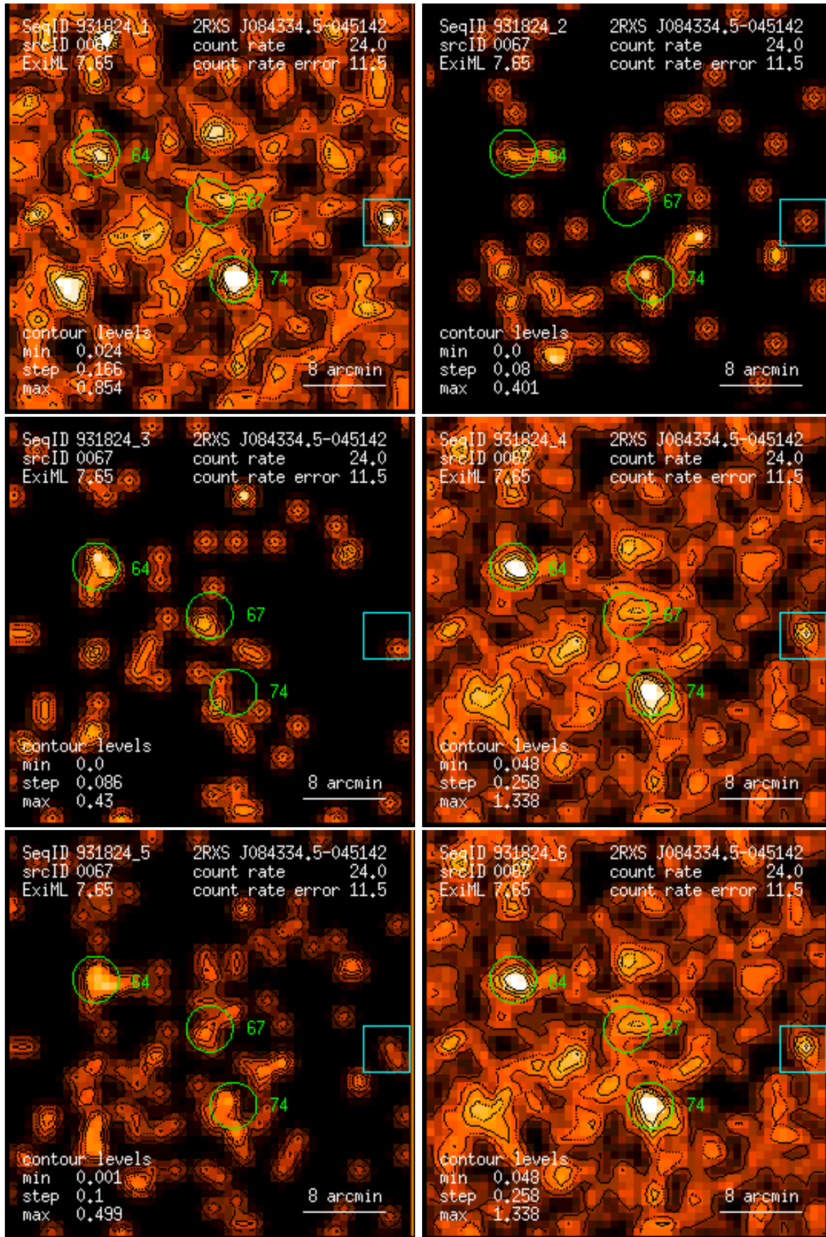
Figure 67: RASS 931824: detection 0067: band rate images, Gaussian filter: (1) PSPC channels 11 – 41, (2) 52 – 90, (3) 91 – 201, (4) 11 – 235, (5) 52 – 201, (6) 11 – 201. Broad band rates in counts/ks. Band rate contour levels in counts/ks/arcmin 2 .
