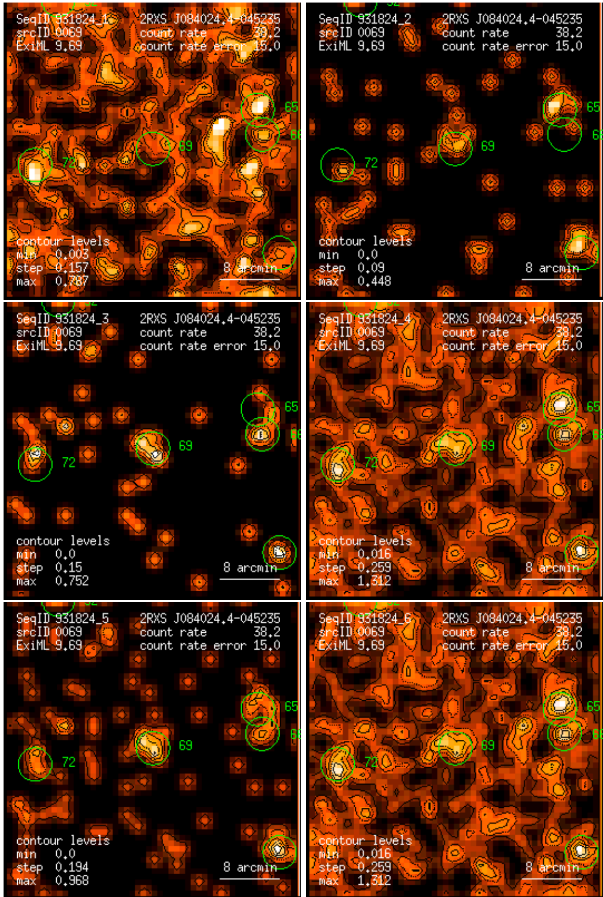
Figure 69: RASS 931824: detection 0069: band rate images, Gaussian filter: (1) PSPC channels 11 – 41, (2) 52 – 90, (3) 91 – 201, (4) 11 – 235, (5) 52 – 201, (6) 11 – 201. Broad band rates in counts/ks. Band rate contour levels in counts/ks/arcmin 2 .
