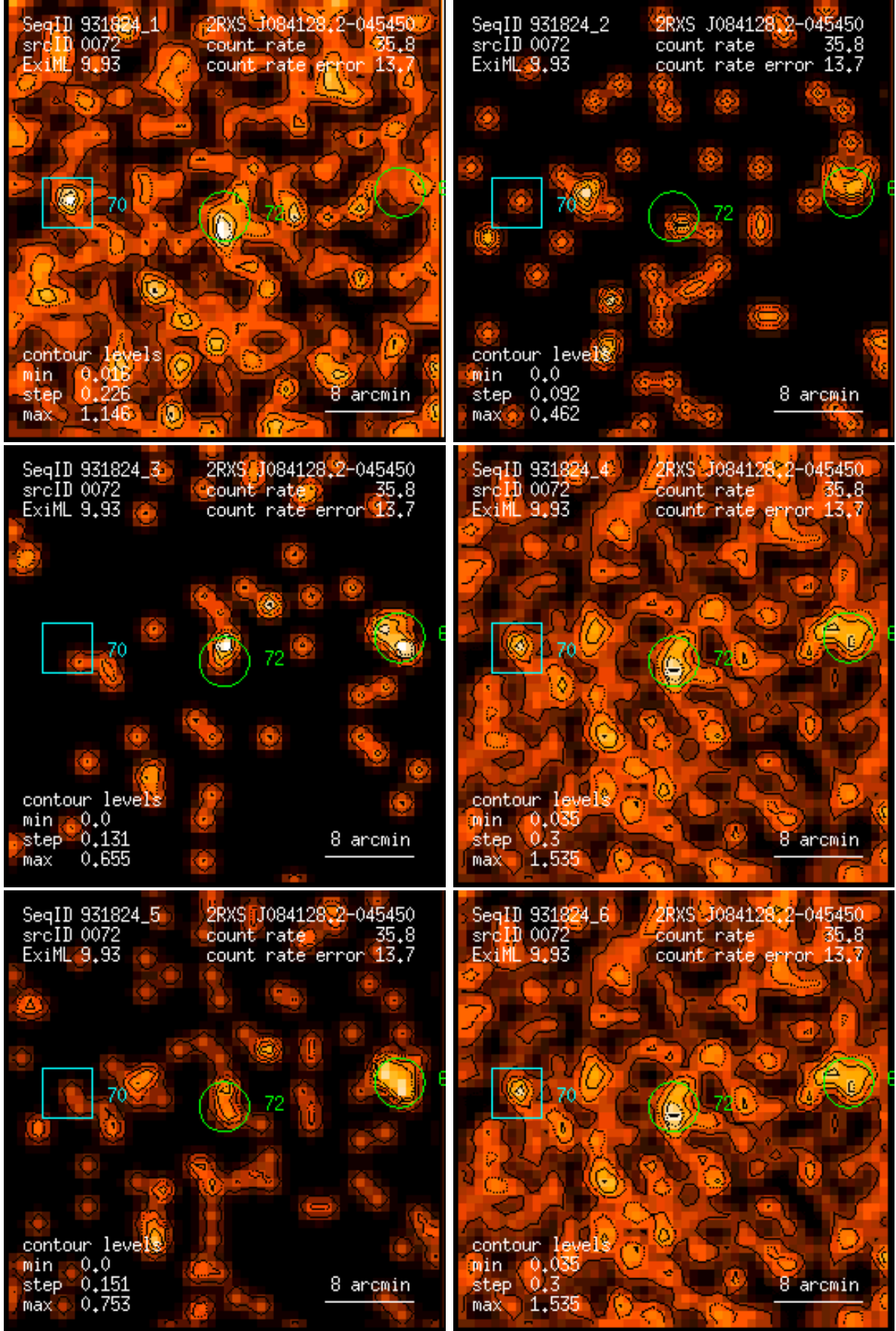
Figure 72: RASS 931824: detection 0072: band rate images, Gaussian filter: (1) PSPC channels 11 – 41, (2) 52 – 90, (3) 91 – 201, (4) 11 – 235, (5) 52 – 201, (6) 11 – 201. Broad band rates in counts/ks. Band rate contour levels in counts/ks/arcmin 2 .
