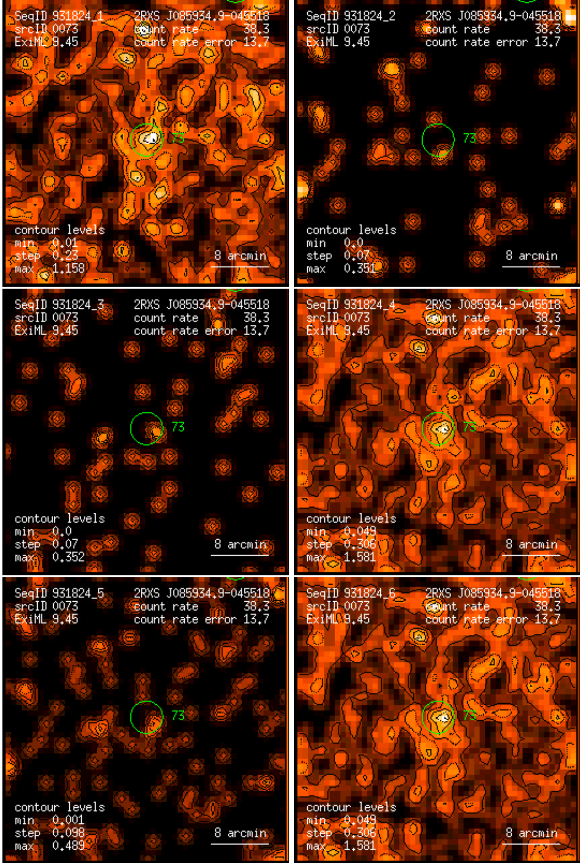
Figure 73: RASS 931824: detection 0073: band rate images, Gaussian filter: (1) PSPC channels 11 – 41, (2) 52 – 90, (3) 91 – 201, (4) 11 – 235, (5) 52 – 201, (6) 11 – 201. Broad band rates in counts/ks. Band rate contour levels in counts/ks/arcmin 2 .
