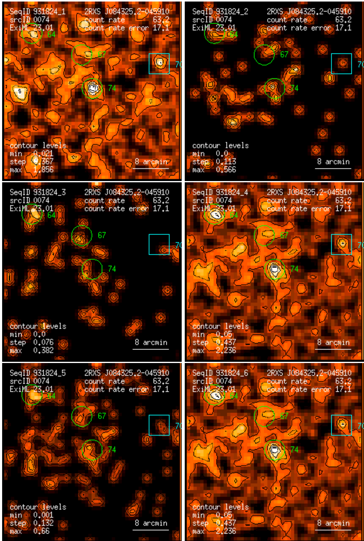
Figure 74: RASS 931824: detection 0074: band rate images, Gaussian filter: (1) PSPC channels 11 – 41, (2) 52 – 90, (3) 91 – 201, (4) 11 – 235, (5) 52 – 201, (6) 11 – 201. Broad band rates in counts/ks. Band rate contour levels in counts/ks/arcmin 2 .
