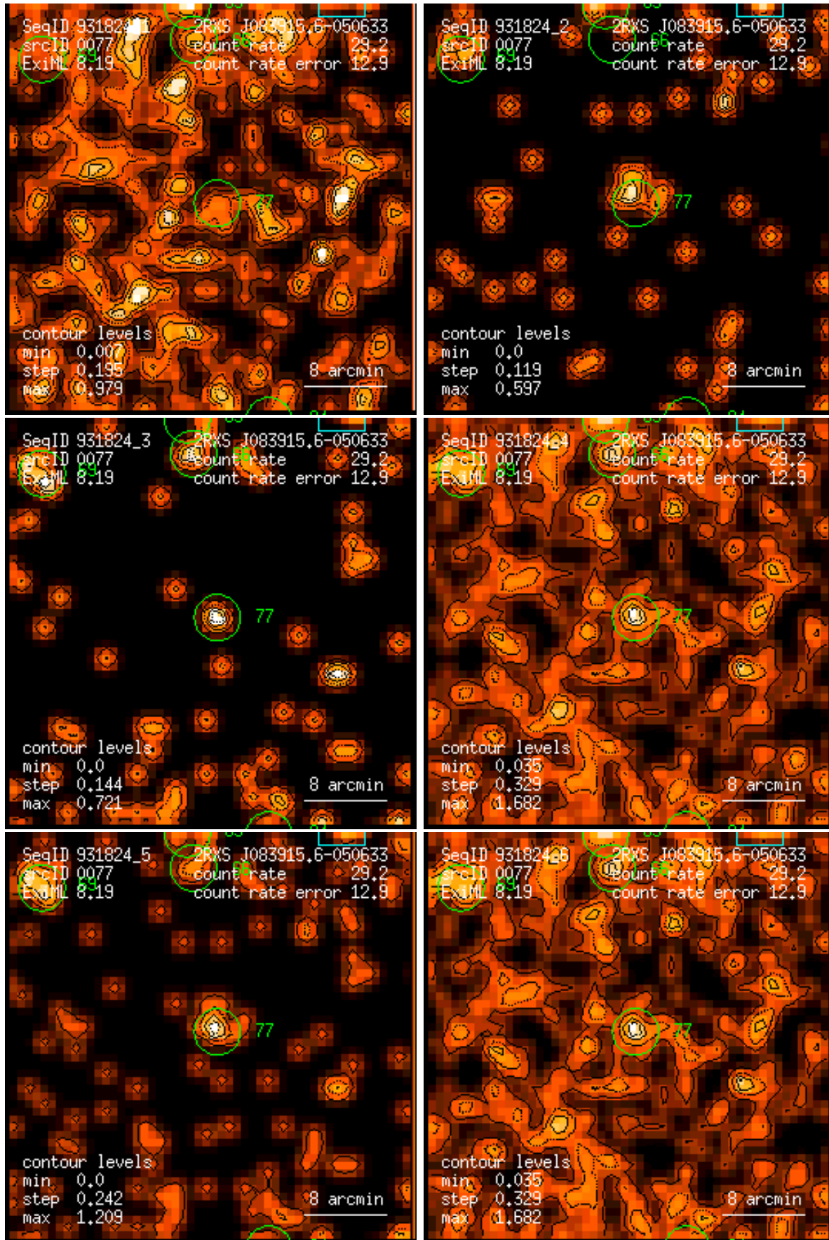
Figure 77: RASS 931824: detection 0077: band rate images, Gaussian filter: (1) PSPC channels 11 – 41, (2) 52 – 90, (3) 91 – 201, (4) 11 – 235, (5) 52 – 201, (6) 11 – 201. Broad band rates in counts/ks. Band rate contour levels in counts/ks/arcmin 2 .
