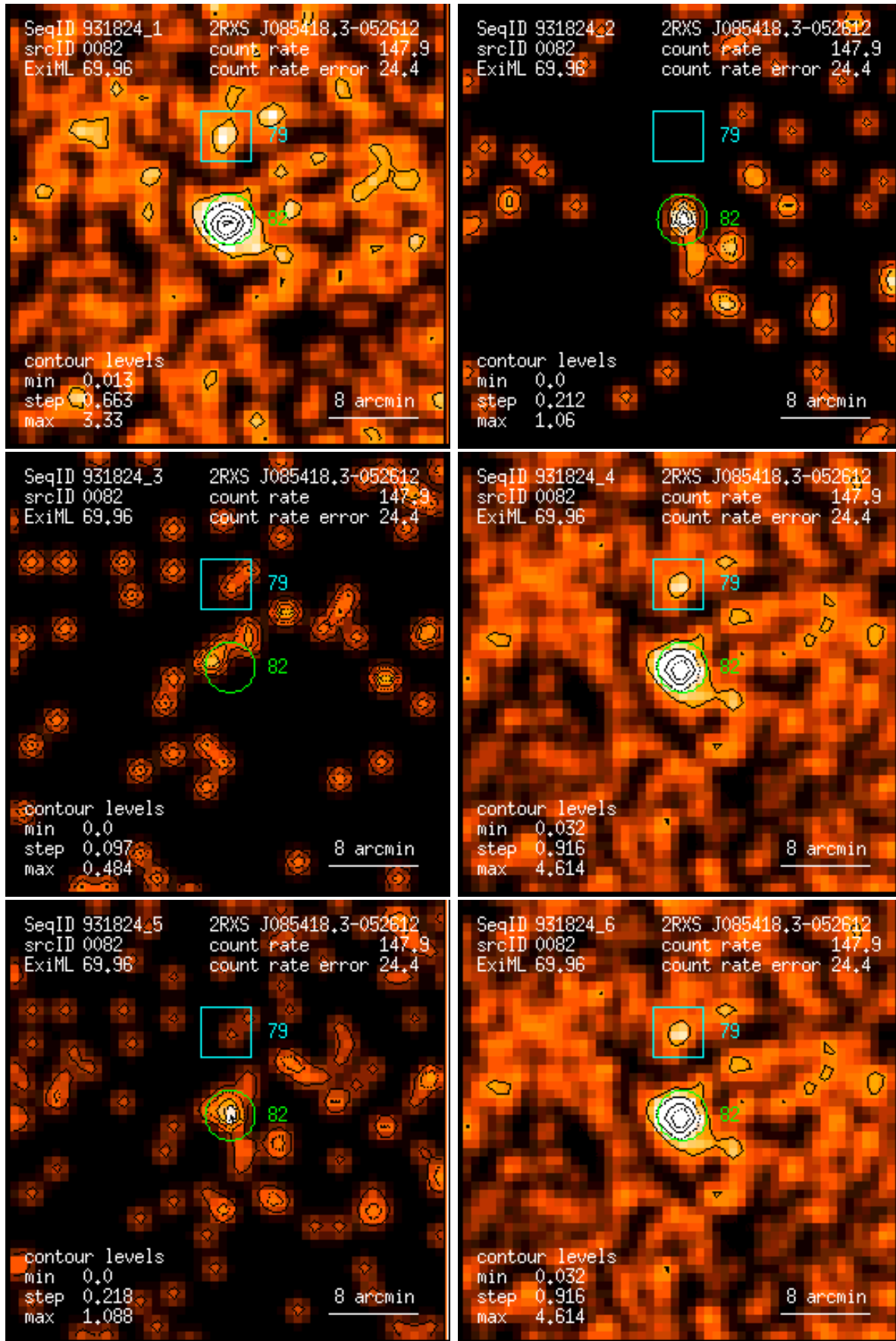
Figure 82: RASS 931824: detection 0082: band rate images, Gaussian filter: (1) PSPC channels 11 – 41, (2) 52 – 90, (3) 91 – 201, (4) 11 – 235, (5) 52 – 201, (6) 11 – 201. Broad band rates in counts/ks. Band rate contour levels in counts/ks/arcmin 2 .
