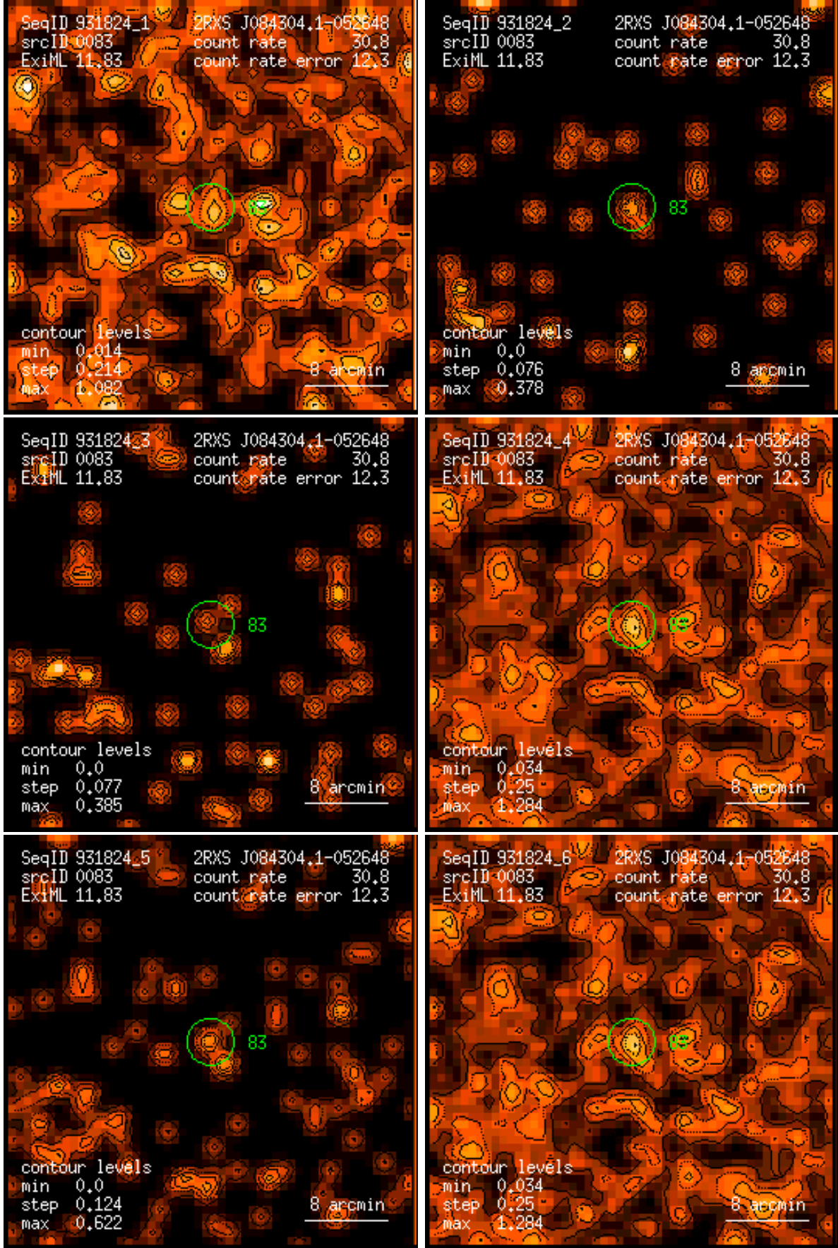
Figure 83: RASS 931824: detection 0083: band rate images, Gaussian filter: (1) PSPC channels 11 – 41, (2) 52 – 90, (3) 91 – 201, (4) 11 – 235, (5) 52 – 201, (6) 11 – 201. Broad band rates in counts/ks. Band rate contour levels in counts/ks/arcmin 2 .
