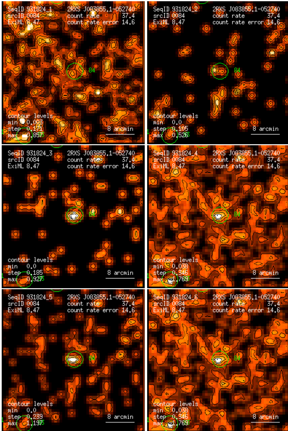
Figure 84: RASS 931824: detection 0084: band rate images, Gaussian filter: (1) PSPC channels 11 – 41, (2) 52 – 90, (3) 91 – 201, (4) 11 – 235, (5) 52 – 201, (6) 11 – 201. Broad band rates in counts/ks. Band rate contour levels in counts/ks/arcmin 2 .
