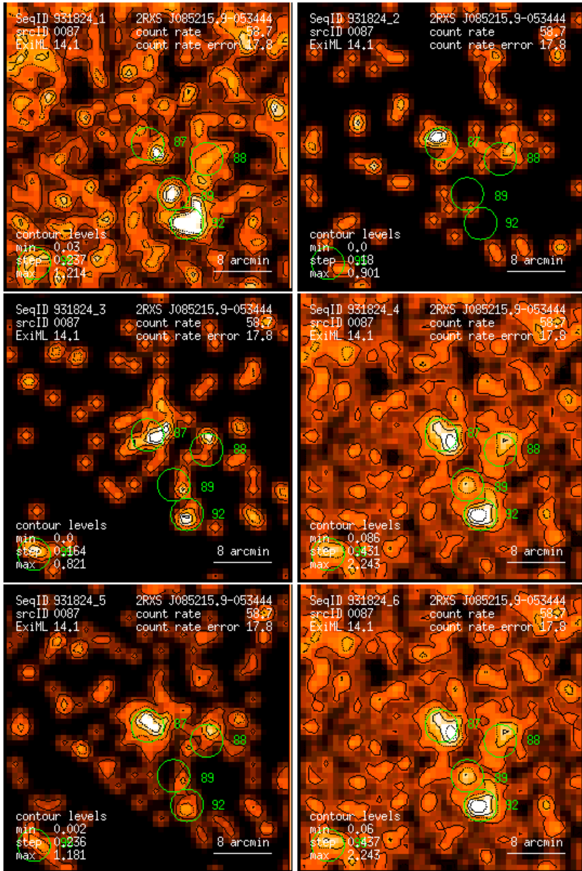
Figure 87: RASS 931824: detection 0087: band rate images, Gaussian filter: (1) PSPC channels 11 – 41, (2) 52 – 90, (3) 91 – 201, (4) 11 – 235, (5) 52 – 201, (6) 11 – 201. Broad band rates in counts/ks. Band rate contour levels in counts/ks/arcmin 2 .
