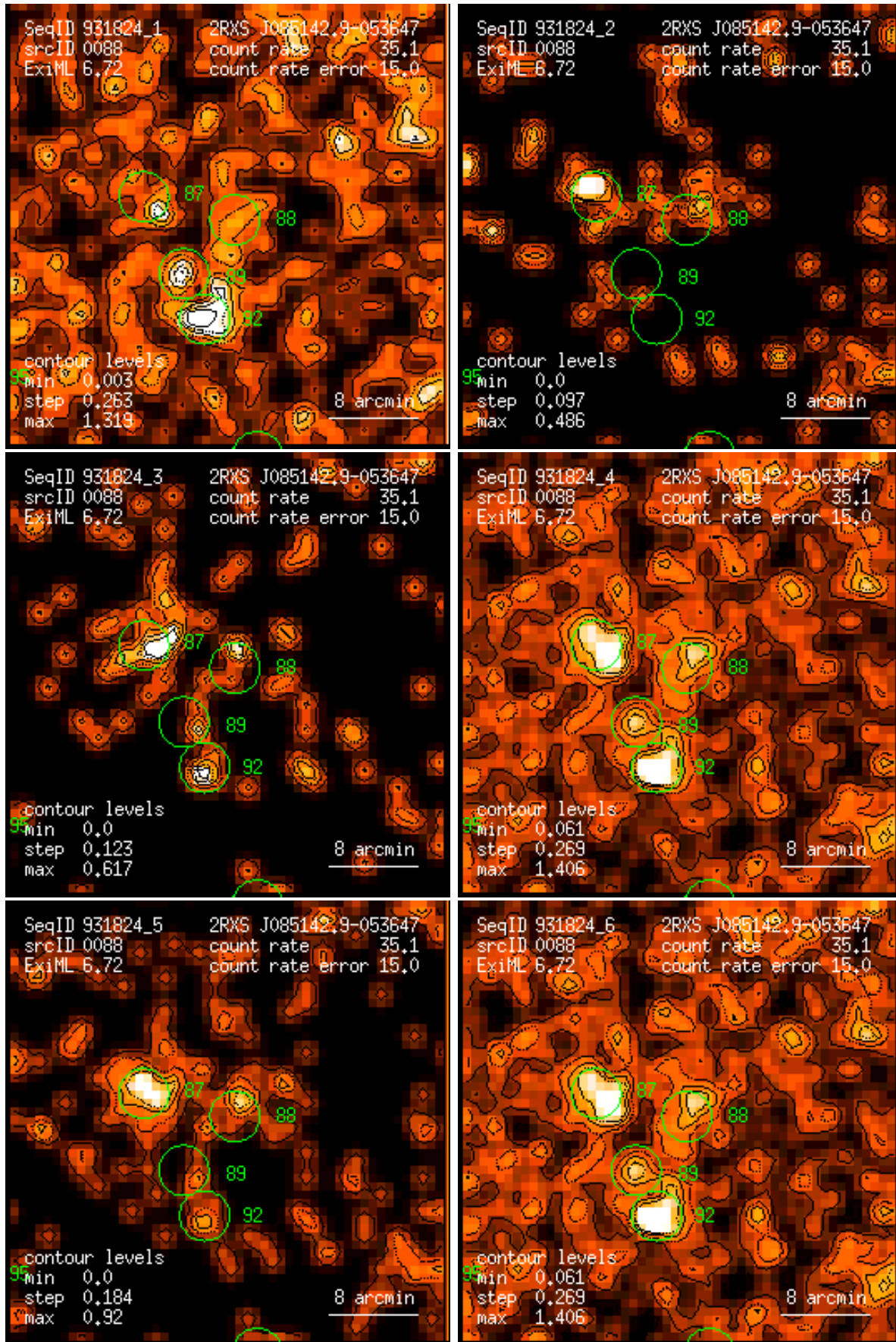
Figure 88: RASS 931824: detection 0088: band rate images, Gaussian filter: (1) PSPC channels 11 – 41, (2) 52 – 90, (3) 91 – 201, (4) 11 – 235, (5) 52 – 201, (6) 11 – 201. Broad band rates in counts/ks. Band rate contour levels in counts/ks/arcmin 2 .
