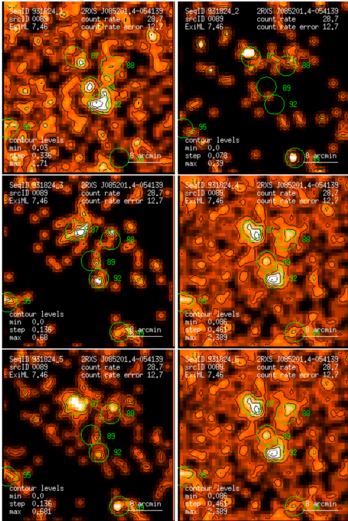
Figure 89: RASS 931824: detection 0089: band rate images, Gaussian filter: (1) PSPC channels 11 – 41, (2) 52 – 90, (3) 91 – 201, (4) 11 – 235, (5) 52 – 201, (6) 11 – 201. Broad band rates in counts/ks. Band rate contour levels in counts/ks/arcmin 2 .
