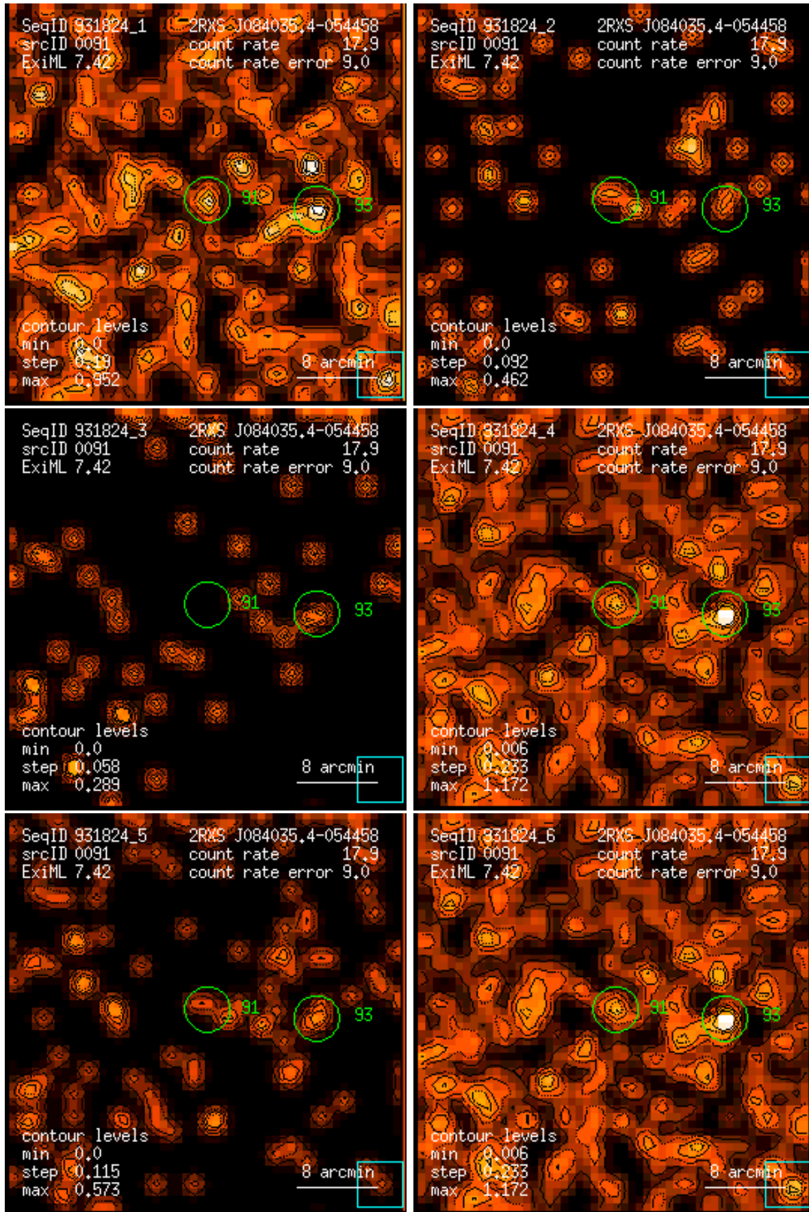
Figure 91: RASS 931824: detection 0091: band rate images, Gaussian filter: (1) PSPC channels 11 – 41, (2) 52 – 90, (3) 91 – 201, (4) 11 – 235, (5) 52 – 201, (6) 11 – 201. Broad band rates in counts/ks. Band rate contour levels in counts/ks/arcmin 2 .
