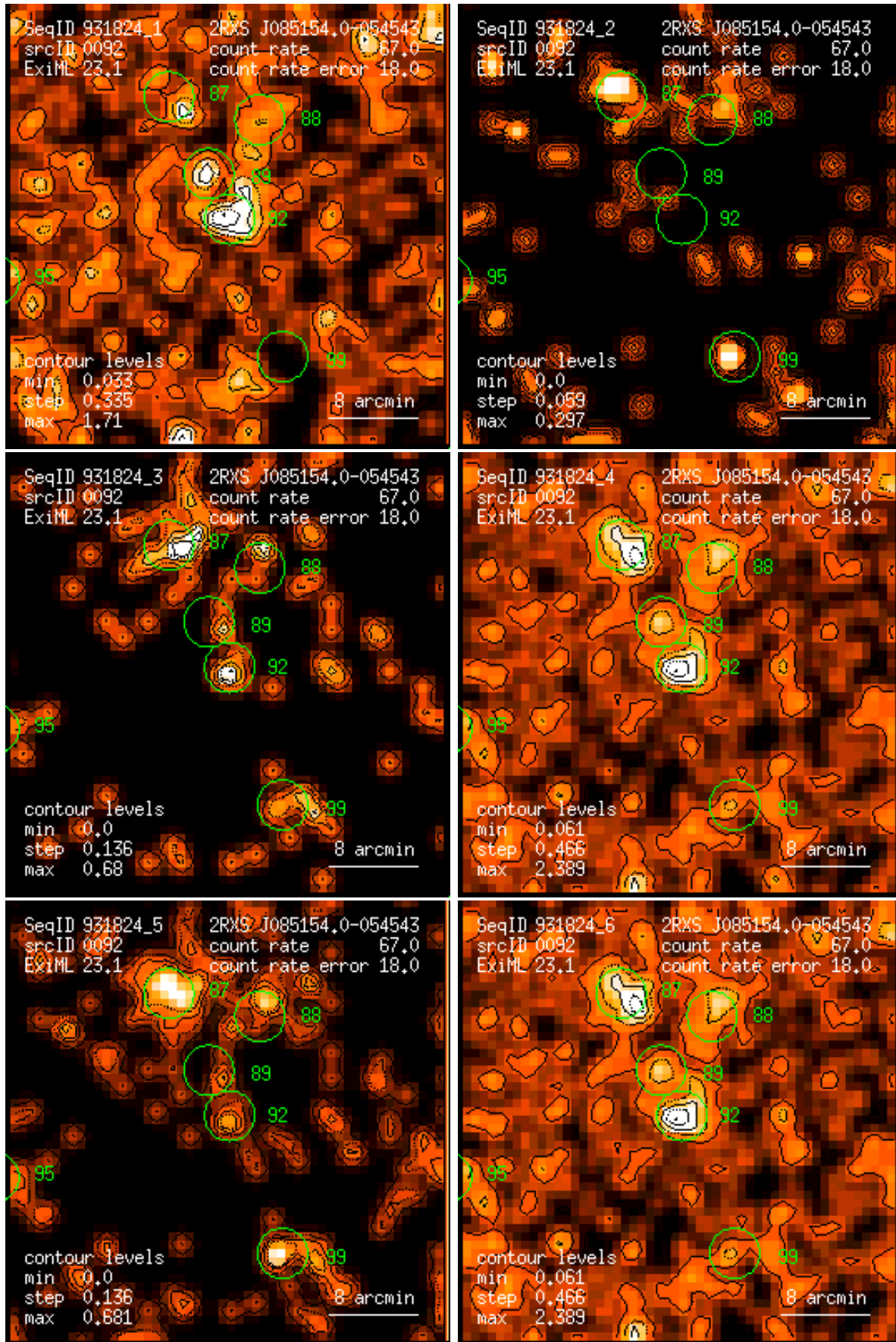
Figure 92: RASS 931824: detection 0092: band rate images, Gaussian filter: (1) PSPC channels 11 – 41, (2) 52 – 90, (3) 91 – 201, (4) 11 – 235, (5) 52 – 201, (6) 11 – 201. Broad band rates in counts/ks. Band rate contour levels in counts/ks/arcmin 2 .
