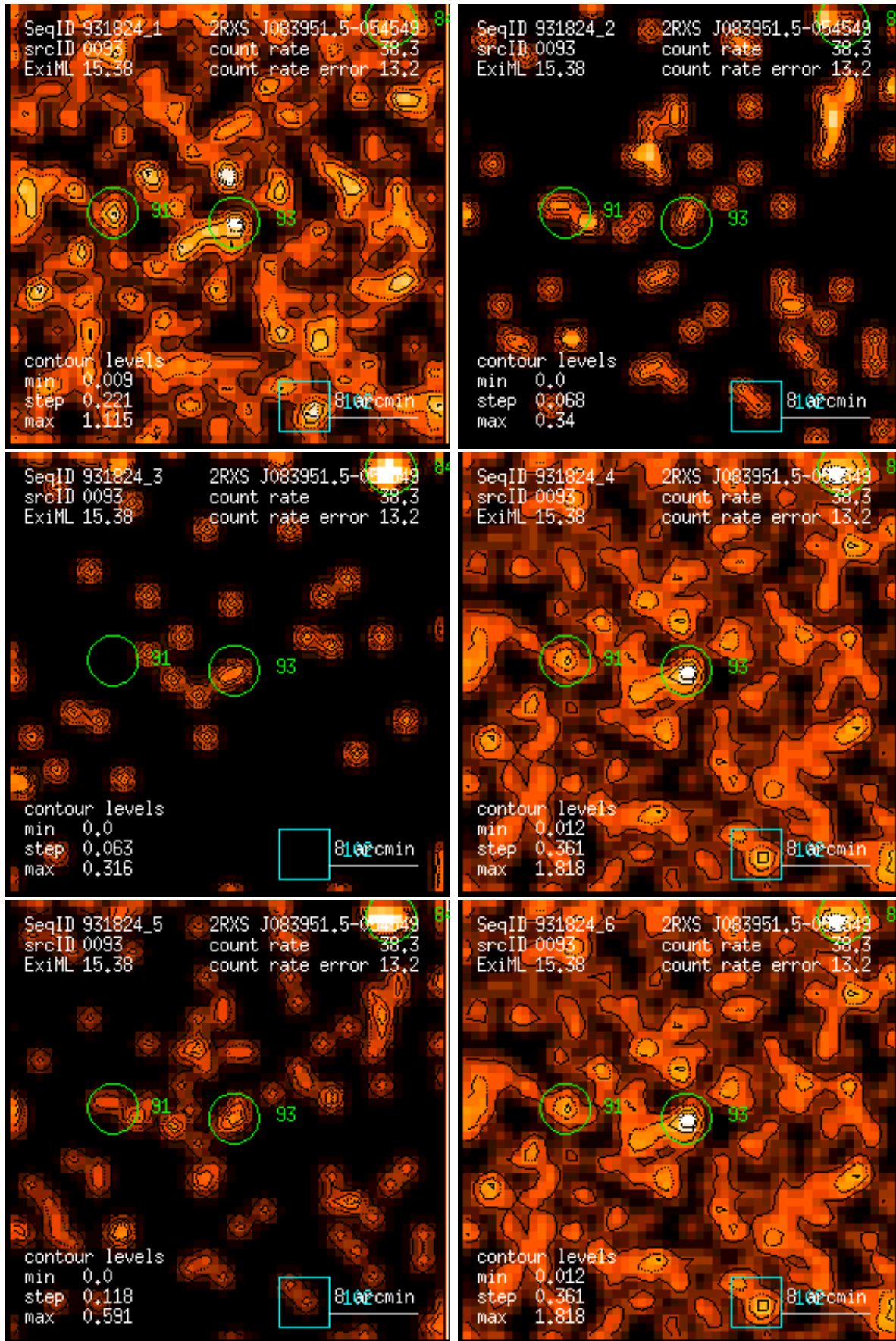
Figure 93: RASS 931824: detection 0093: band rate images, Gaussian filter: (1) PSPC channels 11 – 41, (2) 52 – 90, (3) 91 – 201, (4) 11 – 235, (5) 52 – 201, (6) 11 – 201. Broad band rates in counts/ks. Band rate contour levels in counts/ks/arcmin 2 .
