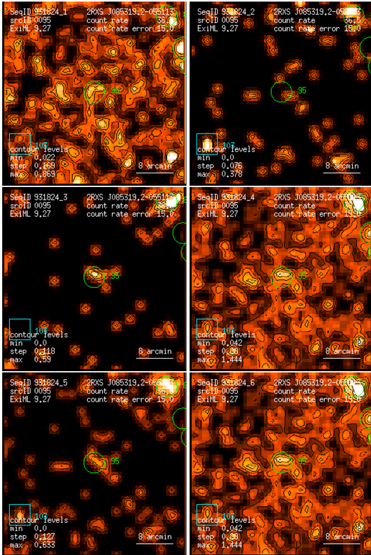
Figure 95: RASS 931824: detection 0095: band rate images, Gaussian filter: (1) PSPC channels 11 – 41, (2) 52 – 90, (3) 91 – 201, (4) 11 – 235, (5) 52 – 201, (6) 11 – 201. Broad band rates in counts/ks. Band rate contour levels in counts/ks/arcmin 2 .
