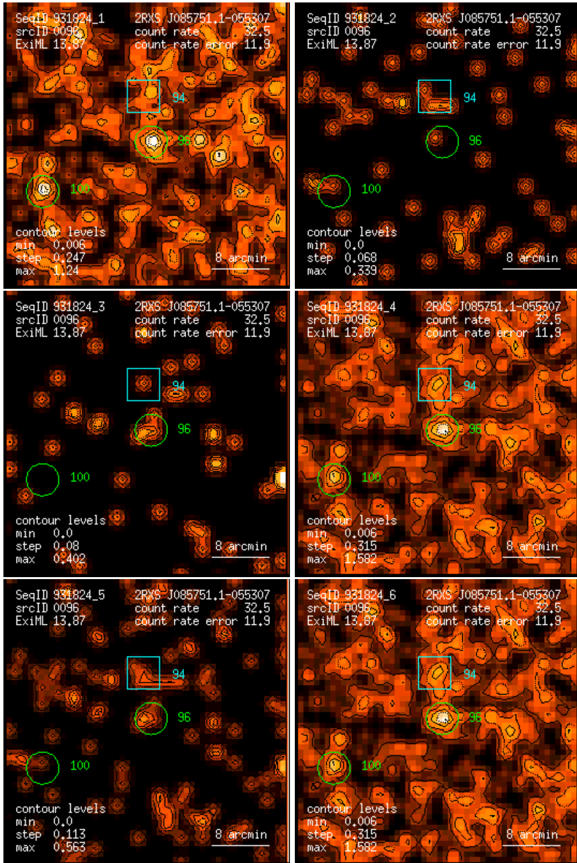
Figure 96: RASS 931824: detection 0096: band rate images, Gaussian filter: (1) PSPC channels 11 – 41, (2) 52 – 90, (3) 91 – 201, (4) 11 – 235, (5) 52 – 201, (6) 11 – 201. Broad band rates in counts/ks. Band rate contour levels in counts/ks/arcmin 2 .
