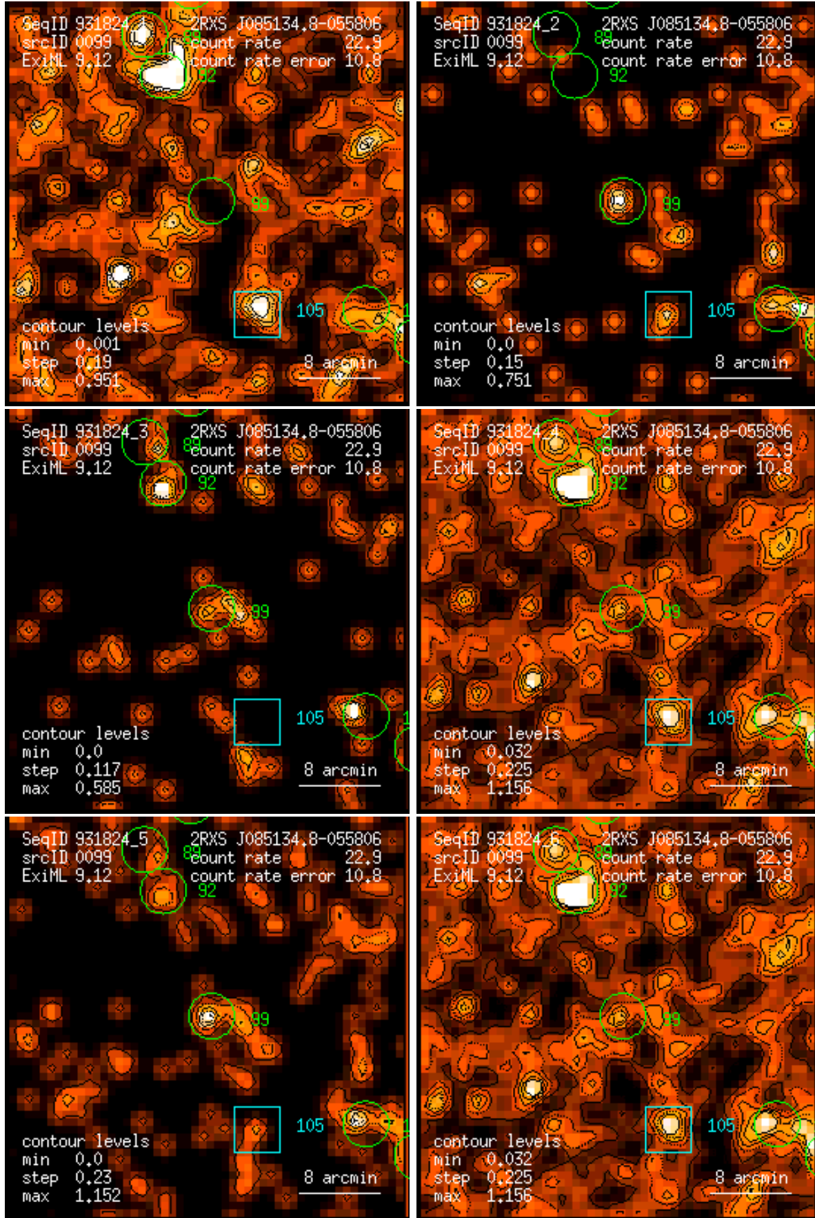
Figure 99: RASS 931824: detection 0099: band rate images, Gaussian filter: (1) PSPC channels 11 – 41, (2) 52 – 90, (3) 91 – 201, (4) 11 – 235, (5) 52 – 201, (6) 11 – 201. Broad band rates in counts/ks. Band rate contour levels in counts/ks/arcmin 2 .
