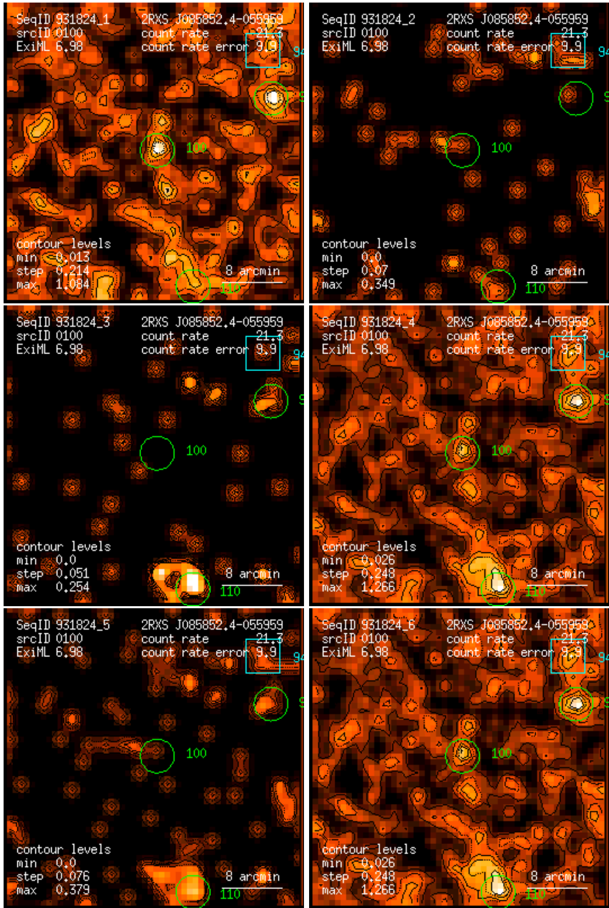
Figure 100: RASS 931824: detection 0100: band rate images, Gaussian filter: (1) PSPC channels 11 – 41, (2) 52 – 90, (3) 91 – 201, (4) 11 – 235, (5) 52 – 201, (6) 11 – 201. Broad band rates in counts/ks. Band rate contour levels in counts/ks/arcmin 2 .
