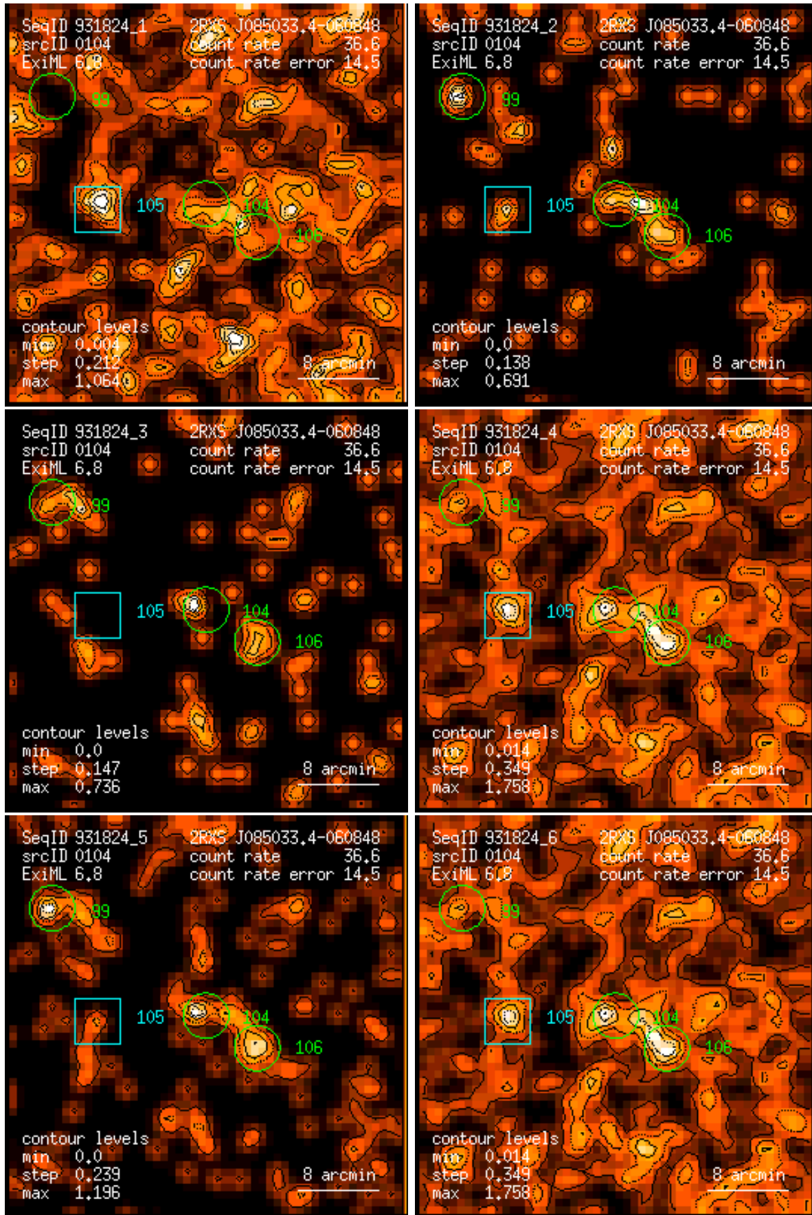
Figure 104: RASS 931824: detection 0104: band rate images, Gaussian filter: (1) PSPC channels 11 – 41, (2) 52 – 90, (3) 91 – 201, (4) 11 – 235, (5) 52 – 201, (6) 11 – 201. Broad band rates in counts/ks. Band rate contour levels in counts/ks/arcmin 2 .
