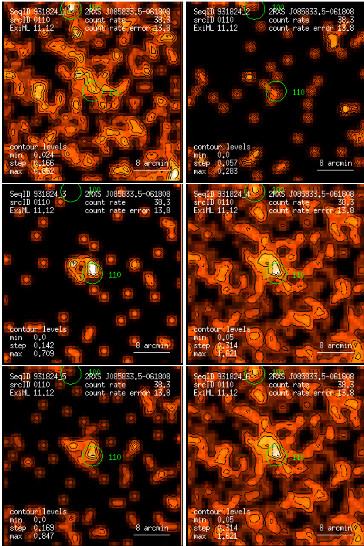
Figure 110: RASS 931824: detection 0110: band rate images, Gaussian filter: (1) PSPC channels 11 – 41, (2) 52 – 90, (3) 91 – 201, (4) 11 – 235, (5) 52 – 201, (6) 11 – 201. Broad band rates in counts/ks. Band rate contour levels in counts/ks/arcmin 2 .
