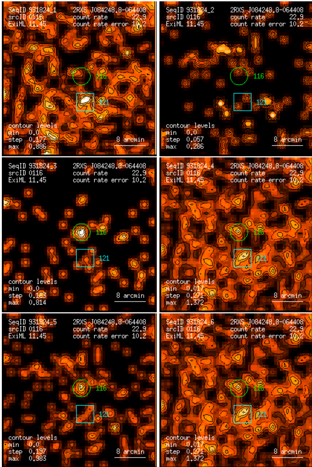
Figure 116: RASS 931824: detection 0116: band rate images, Gaussian filter: (1) PSPC channels 11 – 41, (2) 52 – 90, (3) 91 – 201, (4) 11 – 235, (5) 52 – 201, (6) 11 – 201. Broad band rates in counts/ks. Band rate contour levels in counts/ks/arcmin 2 .
