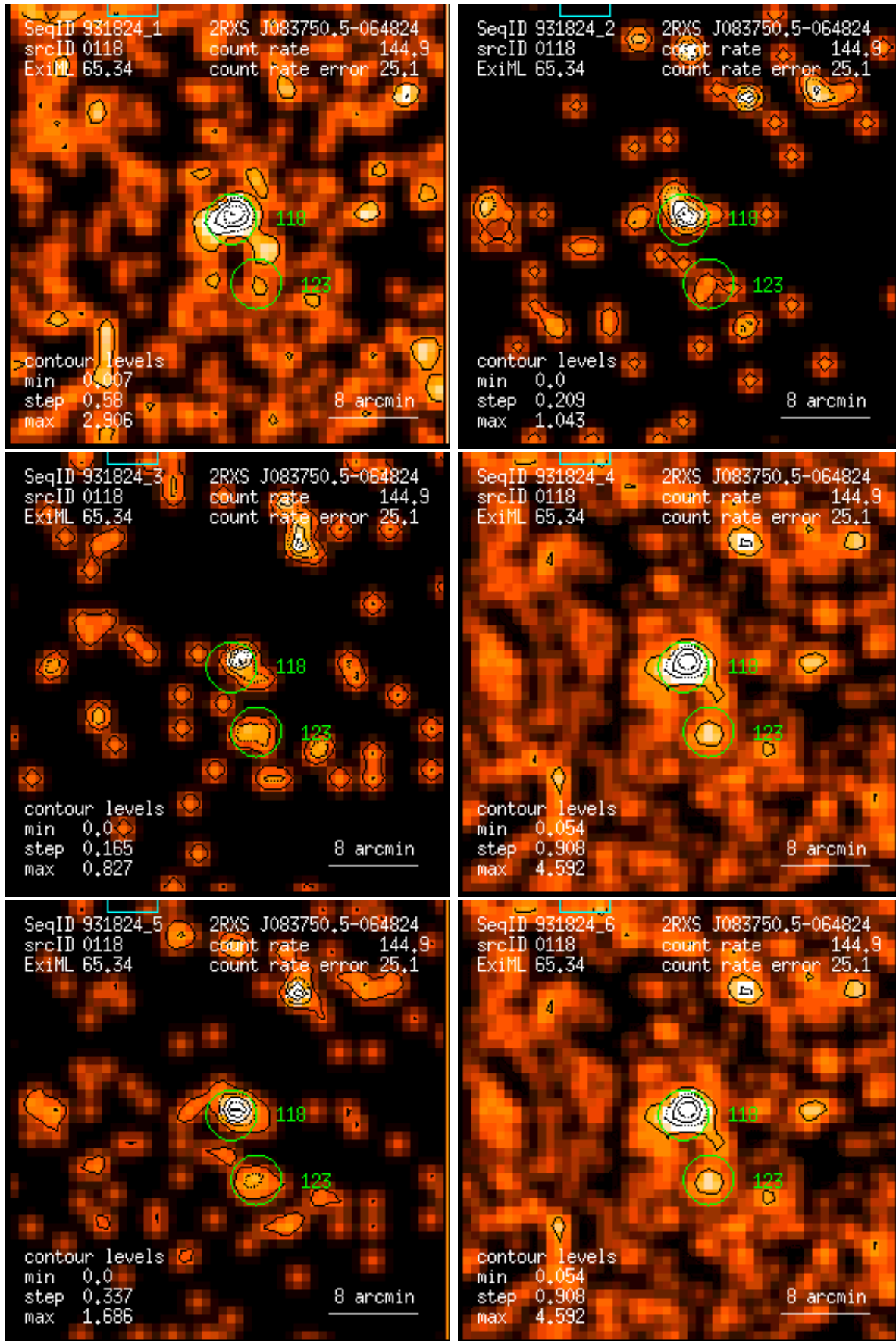
Figure 118: RASS 931824: detection 0118: band rate images, Gaussian filter: (1) PSPC channels 11 – 41, (2) 52 – 90, (3) 91 – 201, (4) 11 – 235, (5) 52 – 201, (6) 11 – 201. Broad band rates in counts/ks. Band rate contour levels in counts/ks/arcmin 2 .
