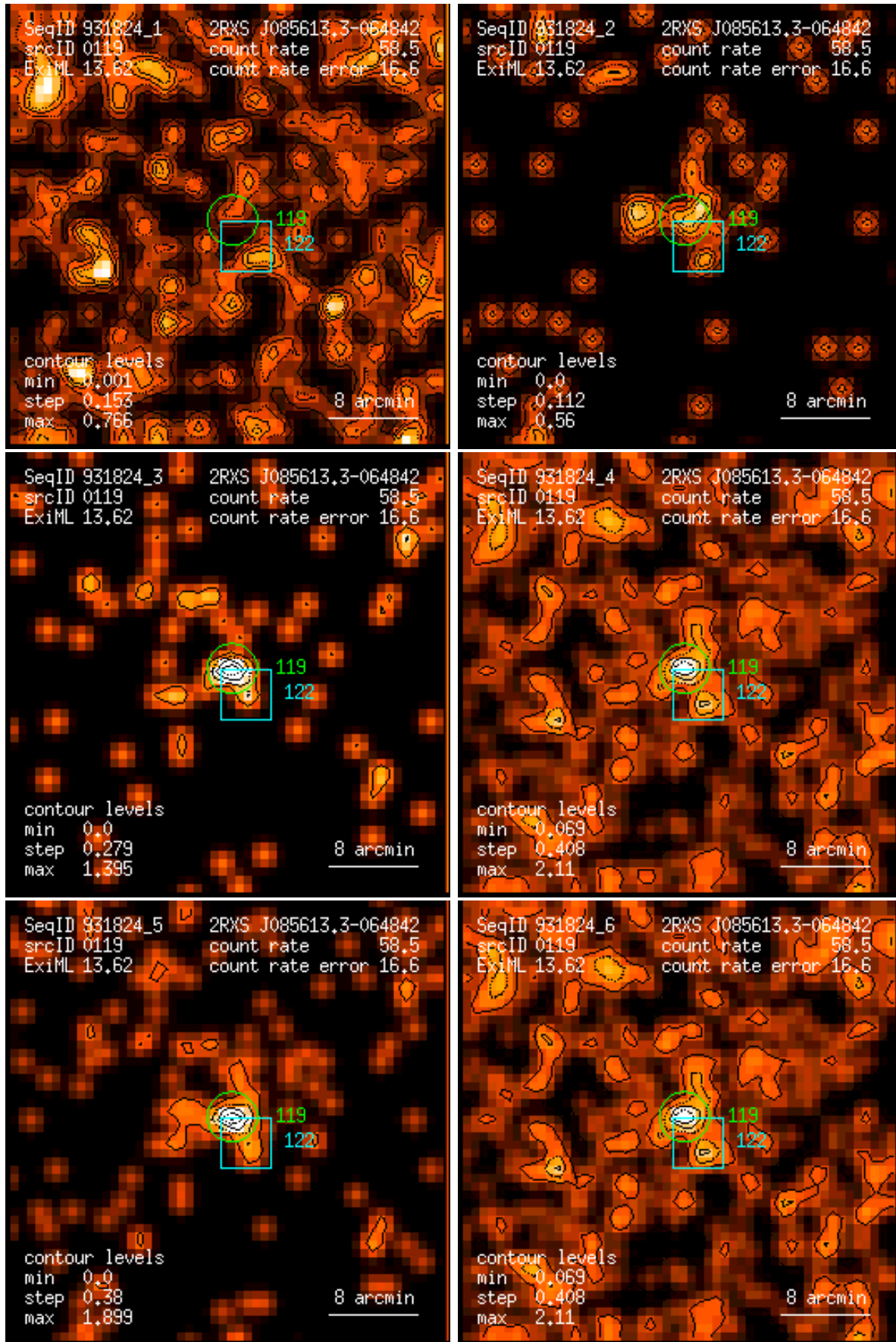
Figure 119: RASS 931824: detection 0119: band rate images, Gaussian filter: (1) PSPC channels 11 – 41, (2) 52 – 90, (3) 91 – 201, (4) 11 – 235, (5) 52 – 201, (6) 11 – 201. Broad band rates in counts/ks. Band rate contour levels in counts/ks/arcmin 2 .
