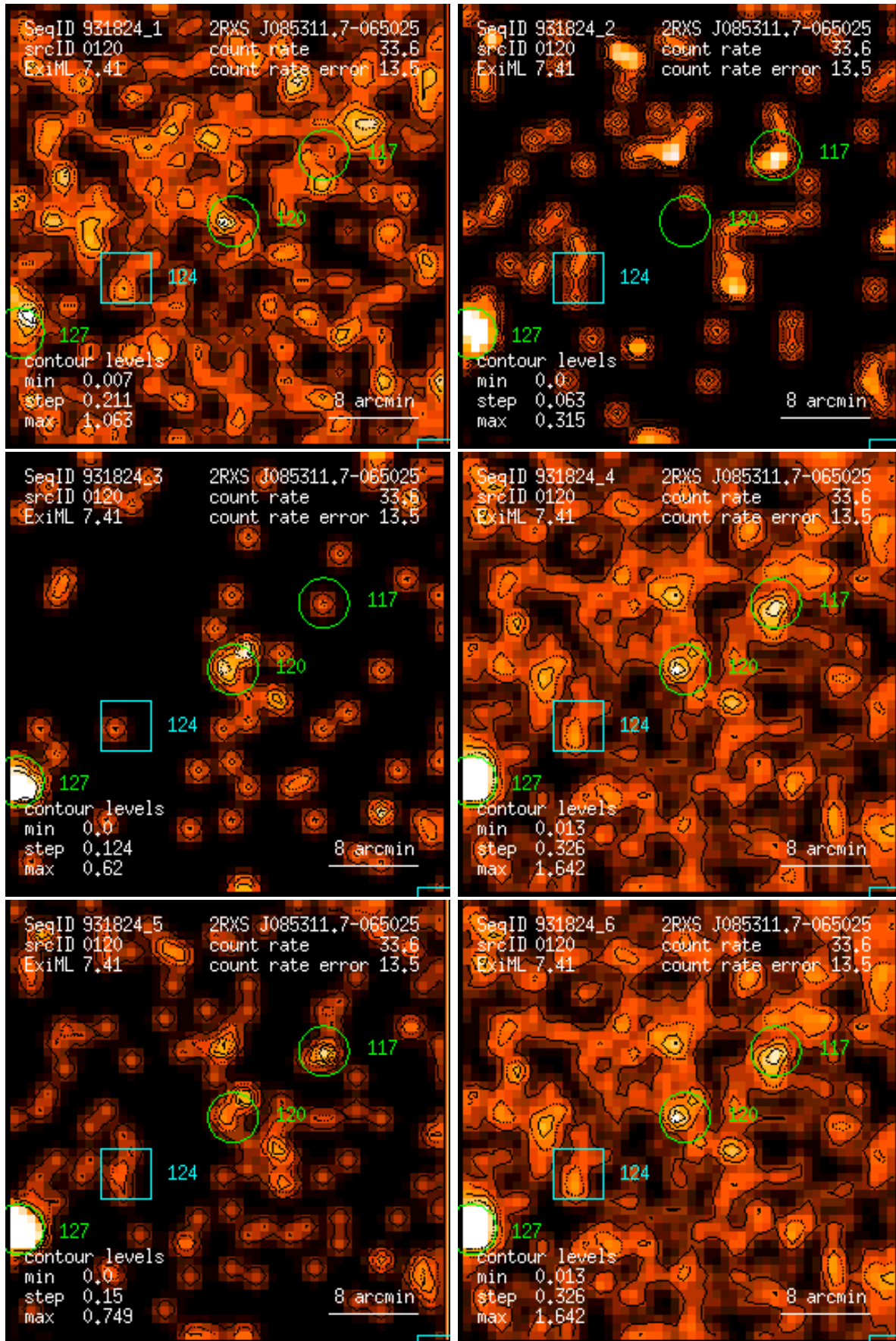
Figure 120: RASS 931824: detection 0120: band rate images, Gaussian filter: (1) PSPC channels 11 – 41, (2) 52 – 90, (3) 91 – 201, (4) 11 – 235, (5) 52 – 201, (6) 11 – 201. Broad band rates in counts/ks. Band rate contour levels in counts/ks/arcmin 2 .
