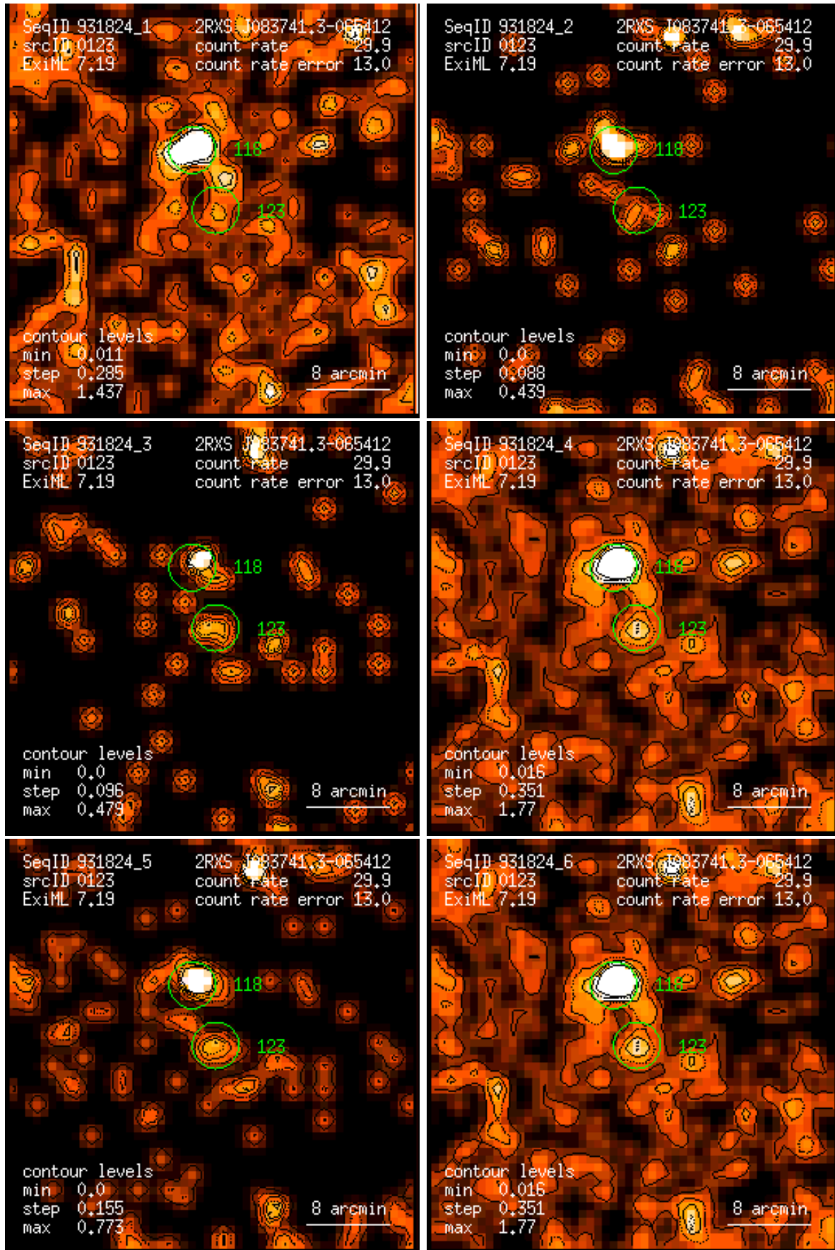
Figure 123: RASS 931824: detection 0123: band rate images, Gaussian filter: (1) PSPC channels 11 – 41, (2) 52 – 90, (3) 91 – 201, (4) 11 – 235, (5) 52 – 201, (6) 11 – 201. Broad band rates in counts/ks. Band rate contour levels in counts/ks/arcmin 2 .
