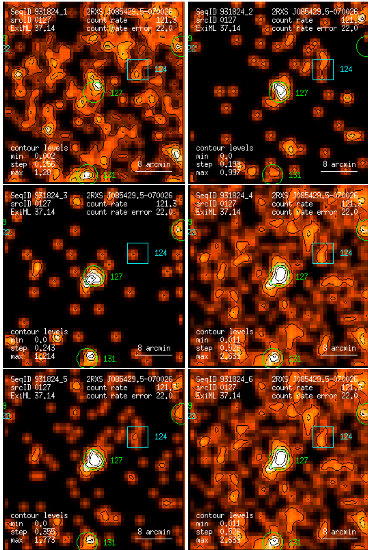
Figure 127: RASS 931824: detection 0127: band rate images, Gaussian filter: (1) PSPC channels 11 – 41, (2) 52 – 90, (3) 91 – 201, (4) 11 – 235, (5) 52 – 201, (6) 11 – 201. Broad band rates in counts/ks. Band rate contour levels in counts/ks/arcmin 2 .
