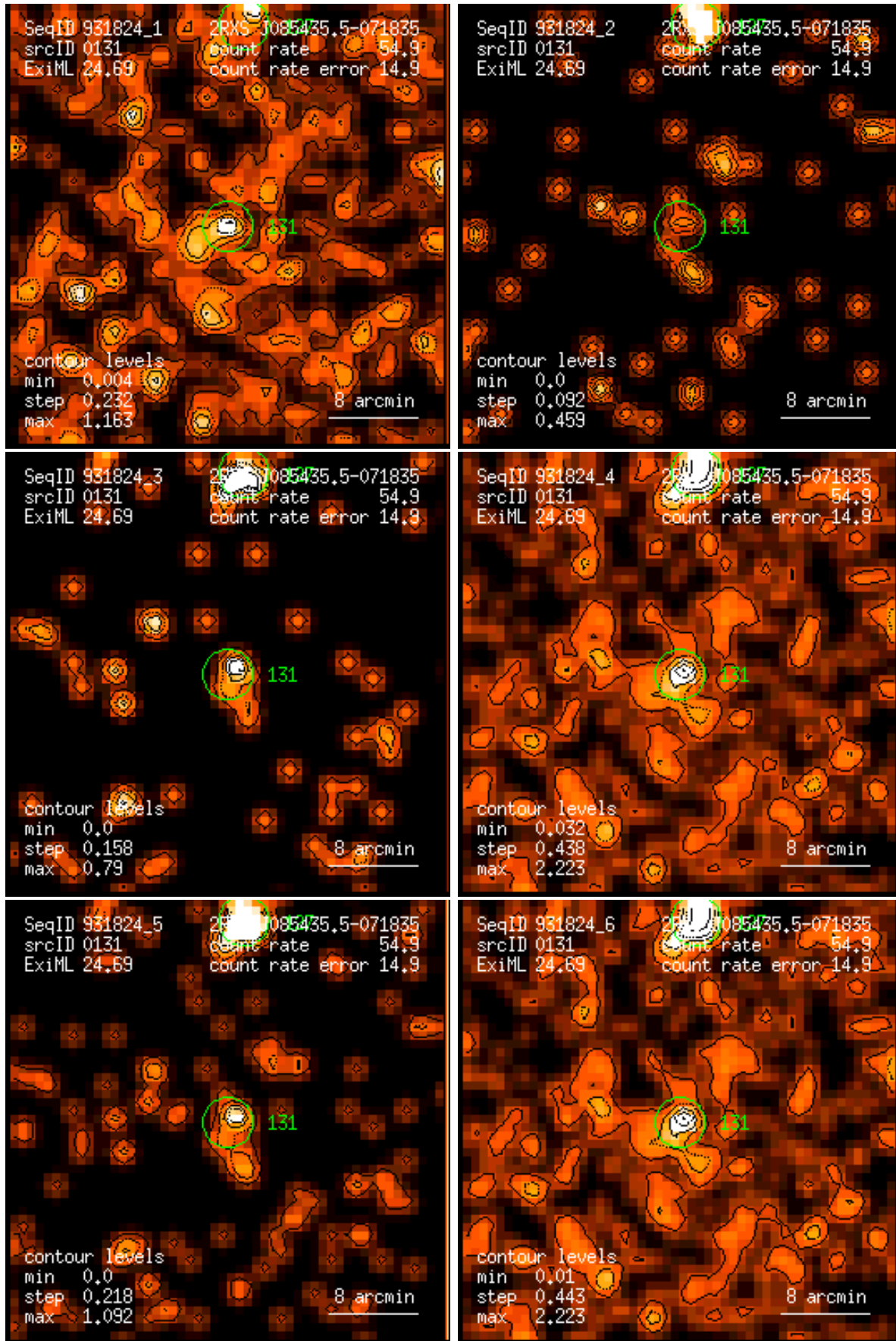
Figure 131: RASS 931824: detection 0131: band rate images, Gaussian filter: (1) PSPC channels 11 – 41, (2) 52 – 90, (3) 91 – 201, (4) 11 – 235, (5) 52 – 201, (6) 11 – 201. Broad band rates in counts/ks. Band rate contour levels in counts/ks/arcmin 2 .
