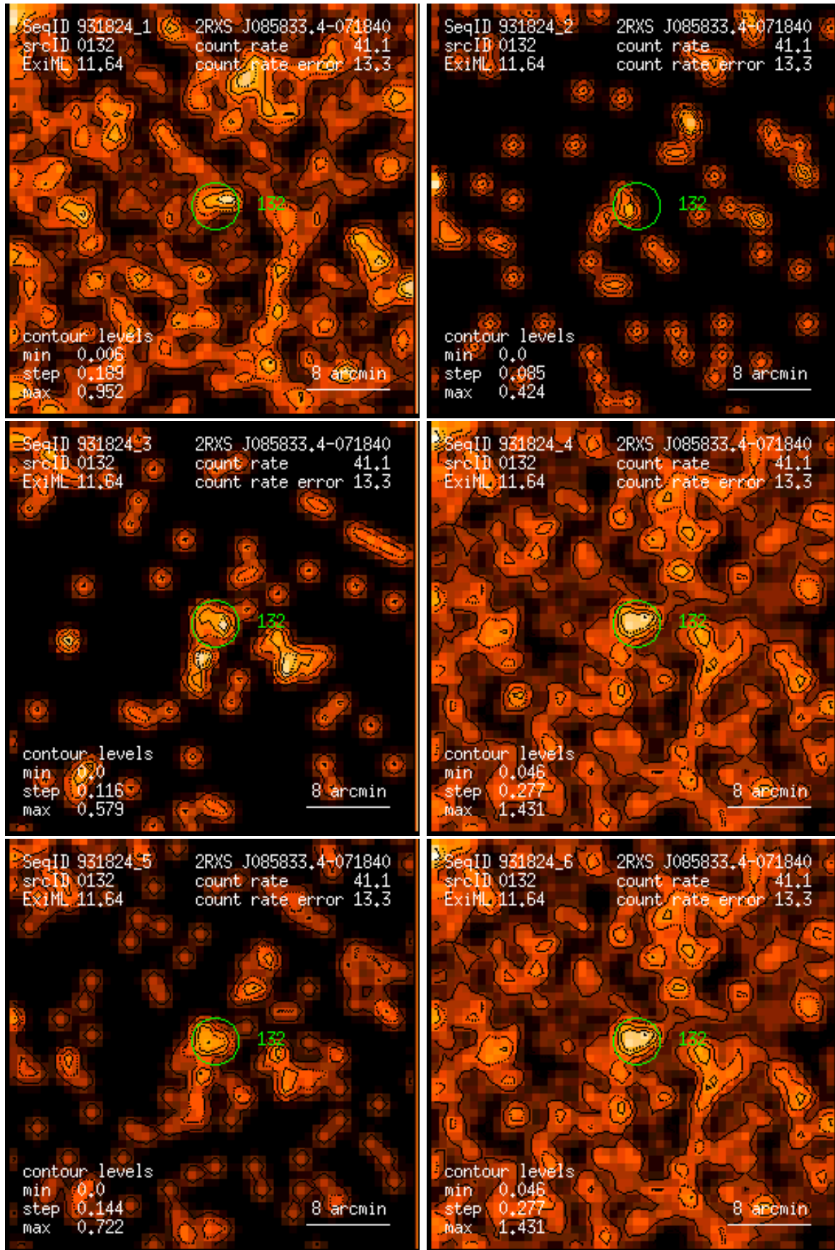
Figure 132: RASS 931824: detection 0132: band rate images, Gaussian filter: (1) PSPC channels 11 – 41, (2) 52 – 90, (3) 91 – 201, (4) 11 – 235, (5) 52 – 201, (6) 11 – 201. Broad band rates in counts/ks. Band rate contour levels in counts/ks/arcmin 2 .
