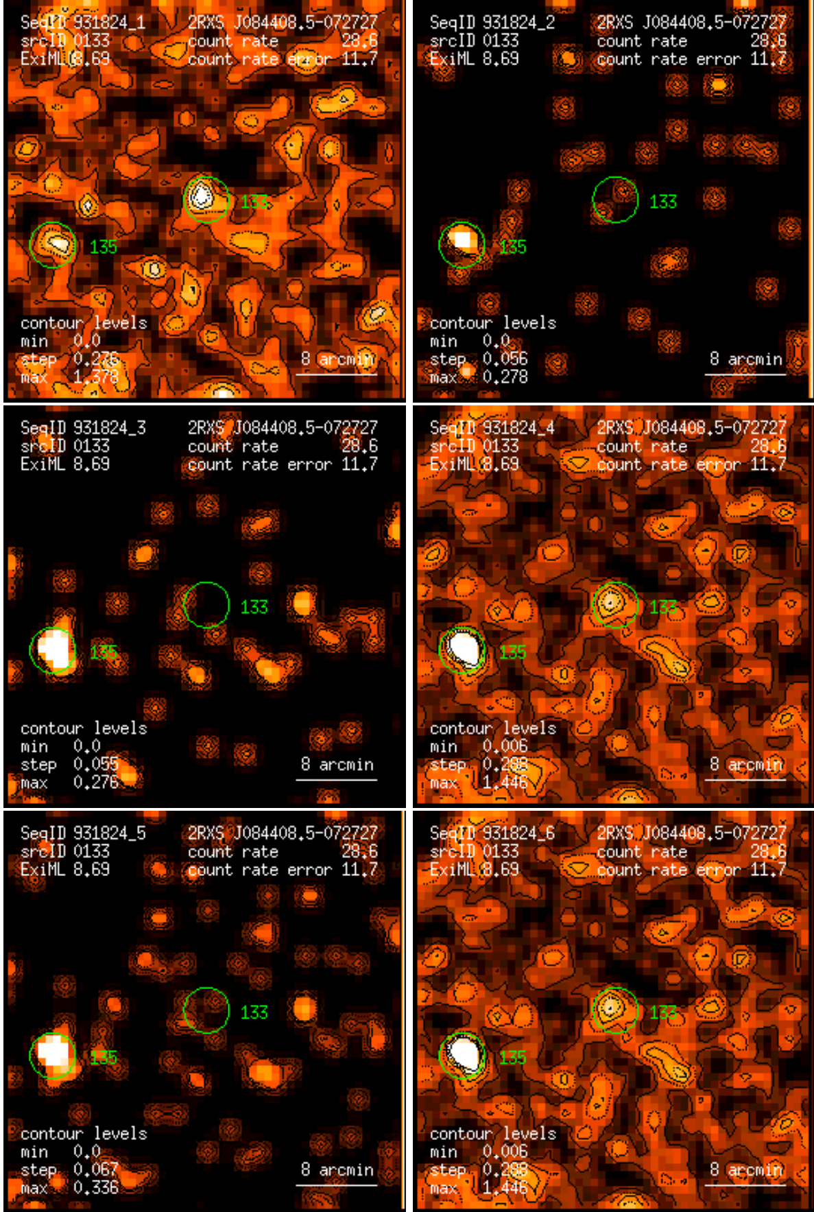
Figure 133: RASS 931824: detection 0133: band rate images, Gaussian filter: (1) PSPC channels 11 – 41, (2) 52 – 90, (3) 91 – 201, (4) 11 – 235, (5) 52 – 201, (6) 11 – 201. Broad band rates in counts/ks. Band rate contour levels in counts/ks/arcmin 2 .
