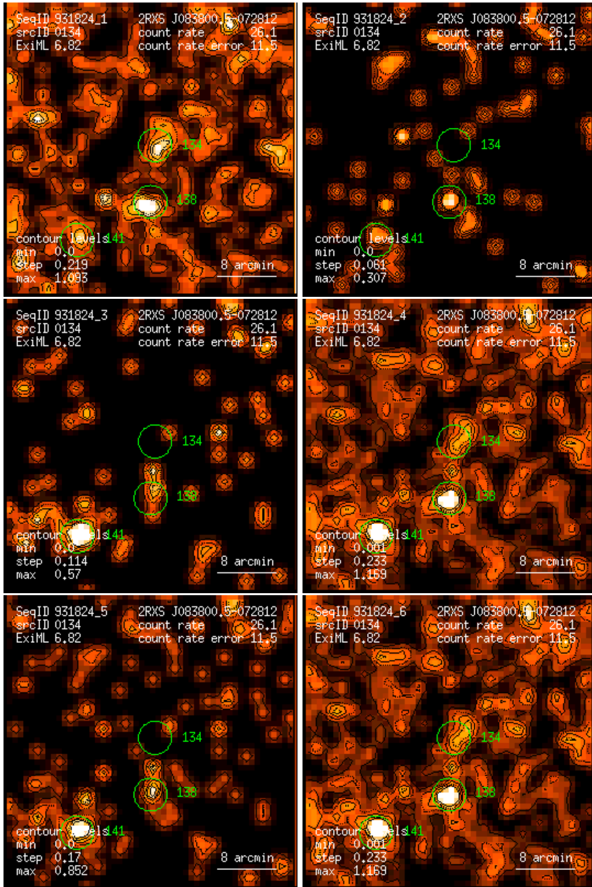
Figure 134: RASS 931824: detection 0134: band rate images, Gaussian filter: (1) PSPC channels 11 – 41, (2) 52 – 90, (3) 91 – 201, (4) 11 – 235, (5) 52 – 201, (6) 11 – 201. Broad band rates in counts/ks. Band rate contour levels in counts/ks/arcmin 2 .
