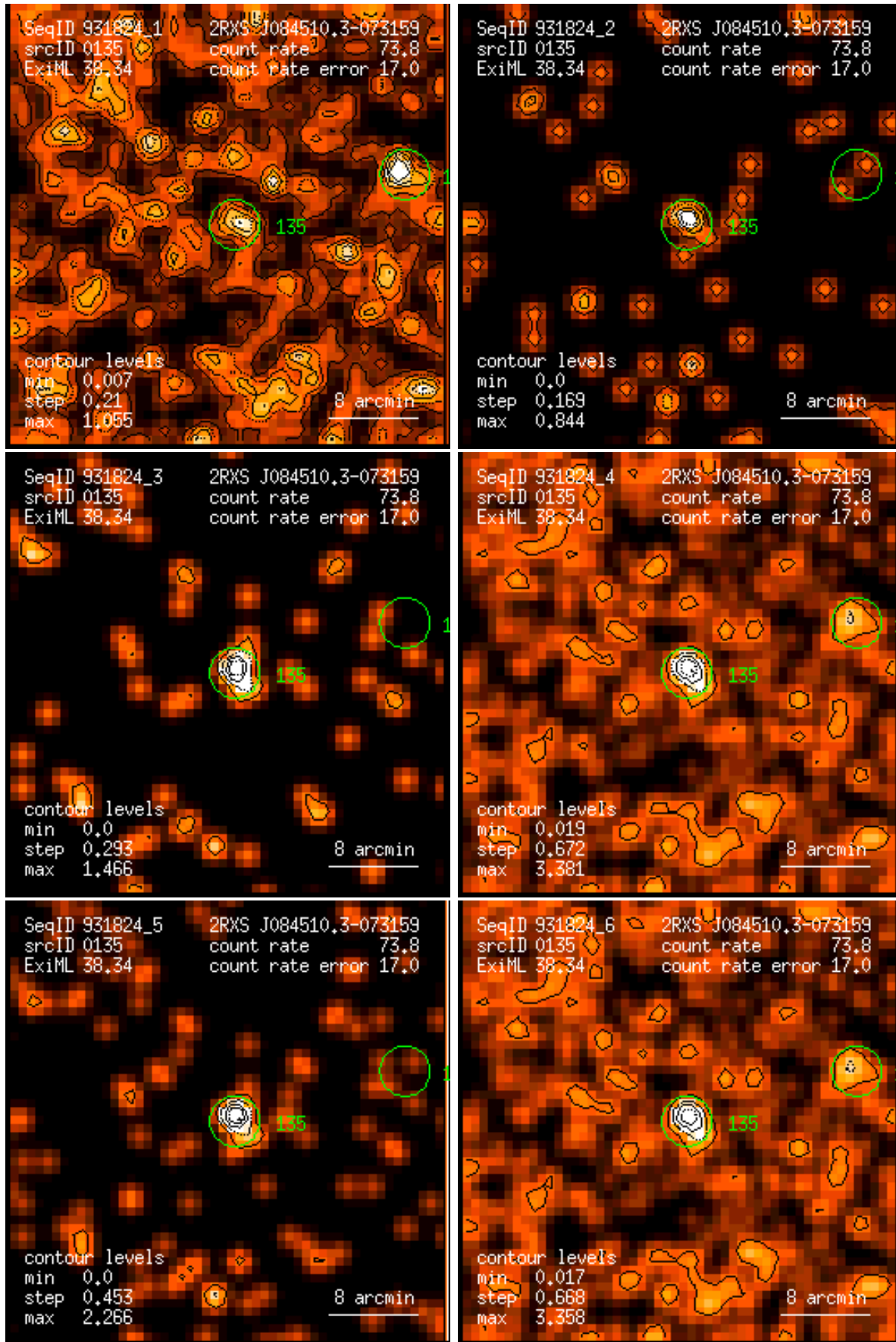
Figure 135: RASS 931824: detection 0135: band rate images, Gaussian filter: (1) PSPC channels 11 – 41, (2) 52 – 90, (3) 91 – 201, (4) 11 – 235, (5) 52 – 201, (6) 11 – 201. Broad band rates in counts/ks. Band rate contour levels in counts/ks/arcmin 2 .
