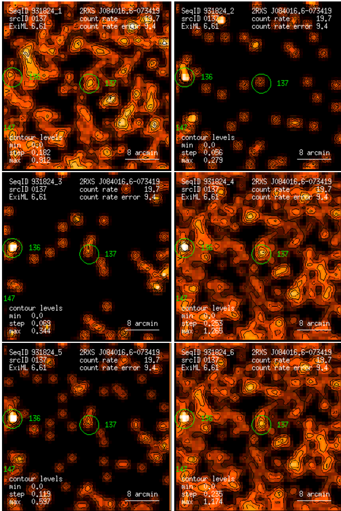
Figure 137: RASS 931824: detection 0137: band rate images, Gaussian filter: (1) PSPC channels 11 – 41, (2) 52 – 90, (3) 91 – 201, (4) 11 – 235, (5) 52 – 201, (6) 11 – 201. Broad band rates in counts/ks. Band rate contour levels in counts/ks/arcmin 2 .
