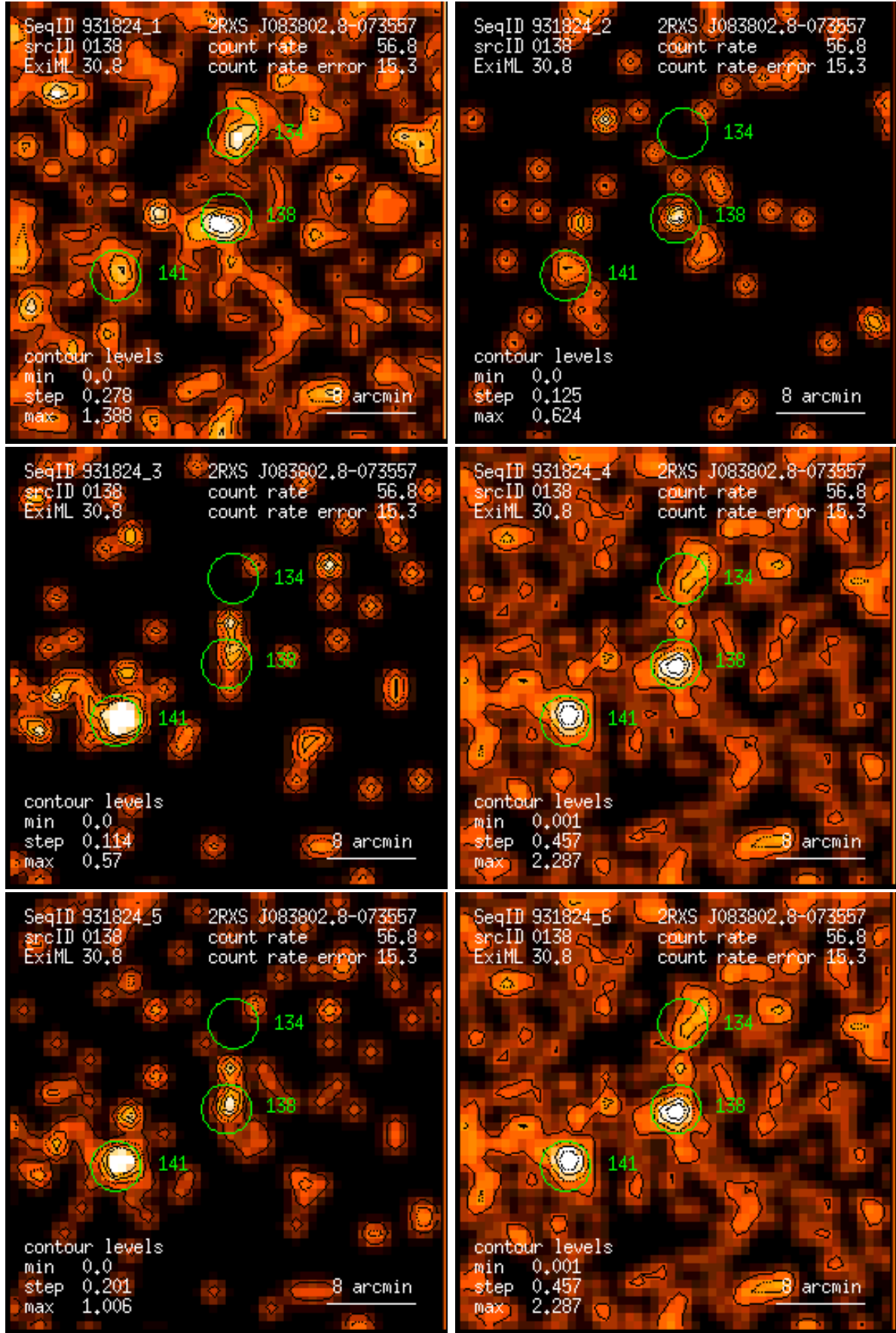
Figure 138: RASS 931824: detection 0138: band rate images, Gaussian filter: (1) PSPC channels 11 – 41, (2) 52 – 90, (3) 91 – 201, (4) 11 – 235, (5) 52 – 201, (6) 11 – 201. Broad band rates in counts/ks. Band rate contour levels in counts/ks/arcmin 2 .
