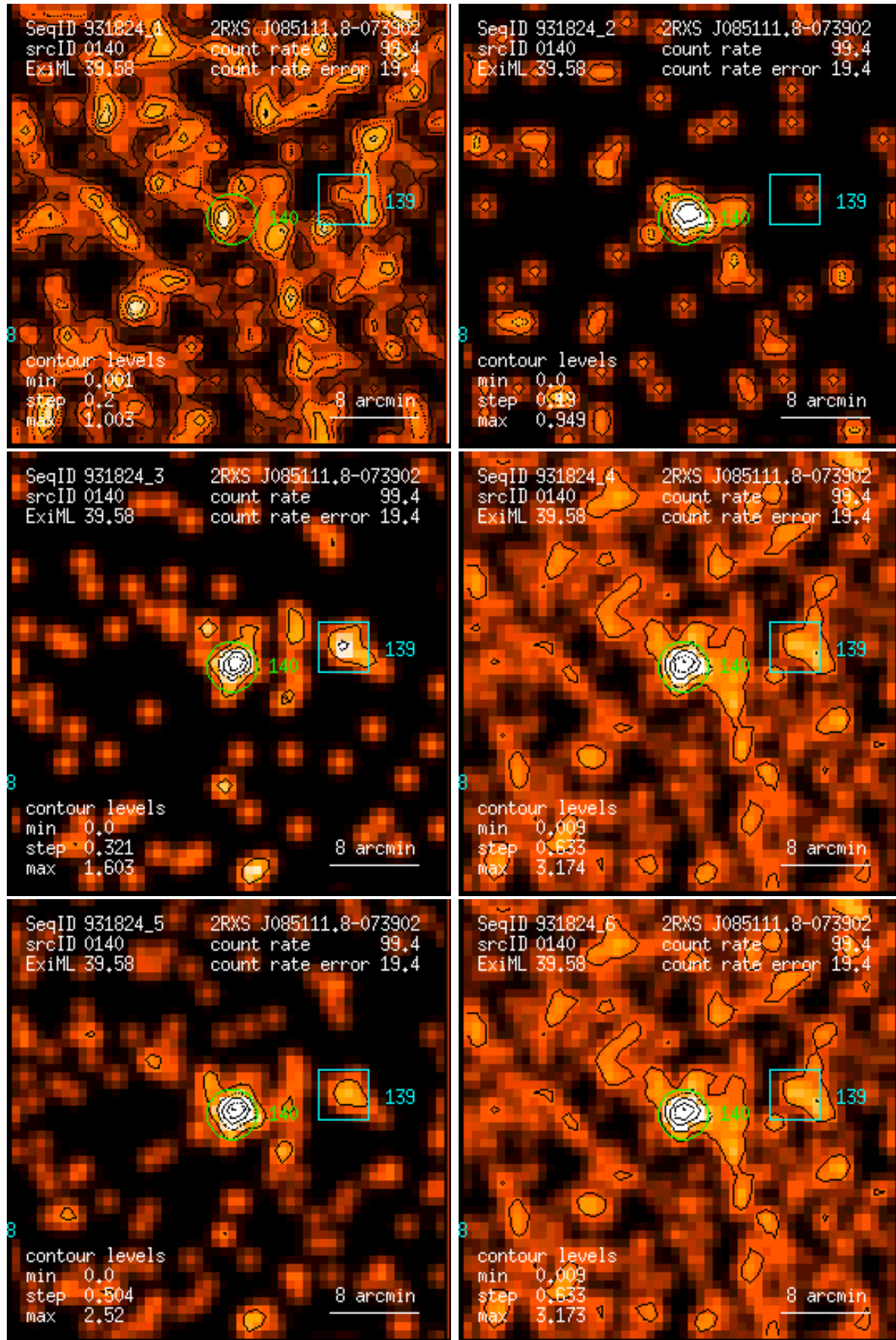
Figure 140: RASS 931824: detection 0140: band rate images, Gaussian filter: (1) PSPC channels 11 – 41, (2) 52 – 90, (3) 91 – 201, (4) 11 – 235, (5) 52 – 201, (6) 11 – 201. Broad band rates in counts/ks. Band rate contour levels in counts/ks/arcmin 2 .
