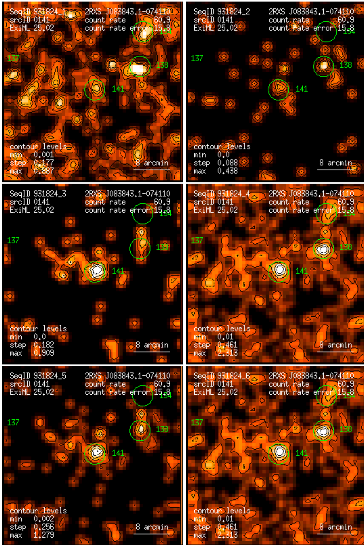
Figure 141: RASS 931824: detection 0141: band rate images, Gaussian filter: (1) PSPC channels 11 – 41, (2) 52 – 90, (3) 91 – 201, (4) 11 – 235, (5) 52 – 201, (6) 11 – 201. Broad band rates in counts/ks. Band rate contour levels in counts/ks/arcmin 2 .
