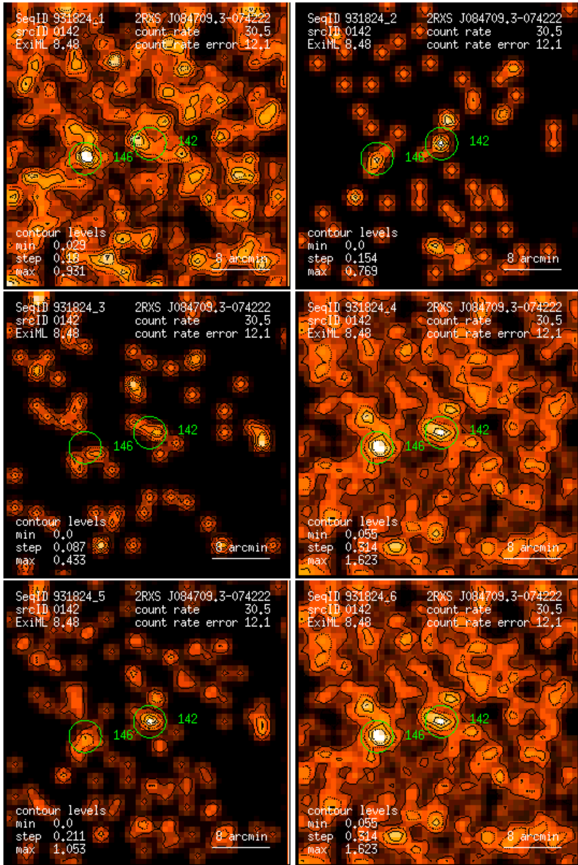
Figure 142: RASS 931824: detection 0142: band rate images, Gaussian filter: (1) PSPC channels 11 – 41, (2) 52 – 90, (3) 91 – 201, (4) 11 – 235, (5) 52 – 201, (6) 11 – 201. Broad band rates in counts/ks. Band rate contour levels in counts/ks/arcmin 2 .
