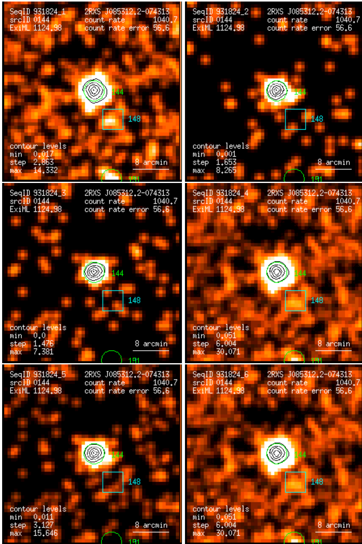
Figure 144: RASS 931824: detection 0144: band rate images, Gaussian filter: (1) PSPC channels 11 – 41, (2) 52 – 90, (3) 91 – 201, (4) 11 – 235, (5) 52 – 201, (6) 11 – 201. Broad band rates in counts/ks. Band rate contour levels in counts/ks/arcmin 2 .
