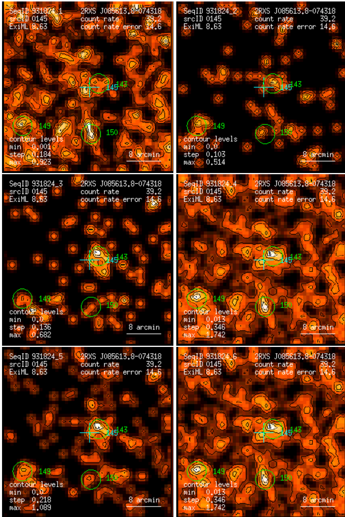
Figure 145: RASS 931824: detection 0145: band rate images, Gaussian filter: (1) PSPC channels 11 – 41, (2) 52 – 90, (3) 91 – 201, (4) 11 – 235, (5) 52 – 201, (6) 11 – 201. Broad band rates in counts/ks. Band rate contour levels in counts/ks/arcmin 2 .
