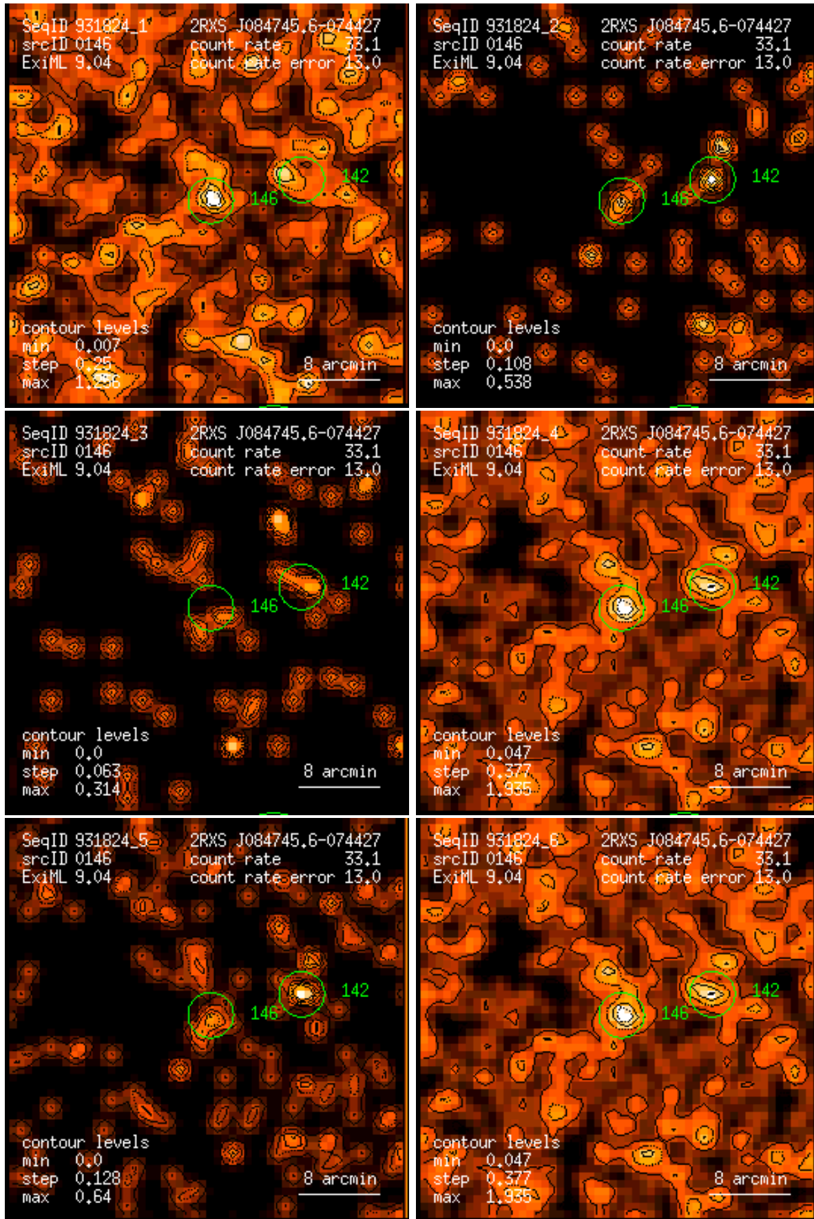
Figure 146: RASS 931824: detection 0146: band rate images, Gaussian filter: (1) PSPC channels 11 – 41, (2) 52 – 90, (3) 91 – 201, (4) 11 – 235, (5) 52 – 201, (6) 11 – 201. Broad band rates in counts/ks. Band rate contour levels in counts/ks/arcmin 2 .
