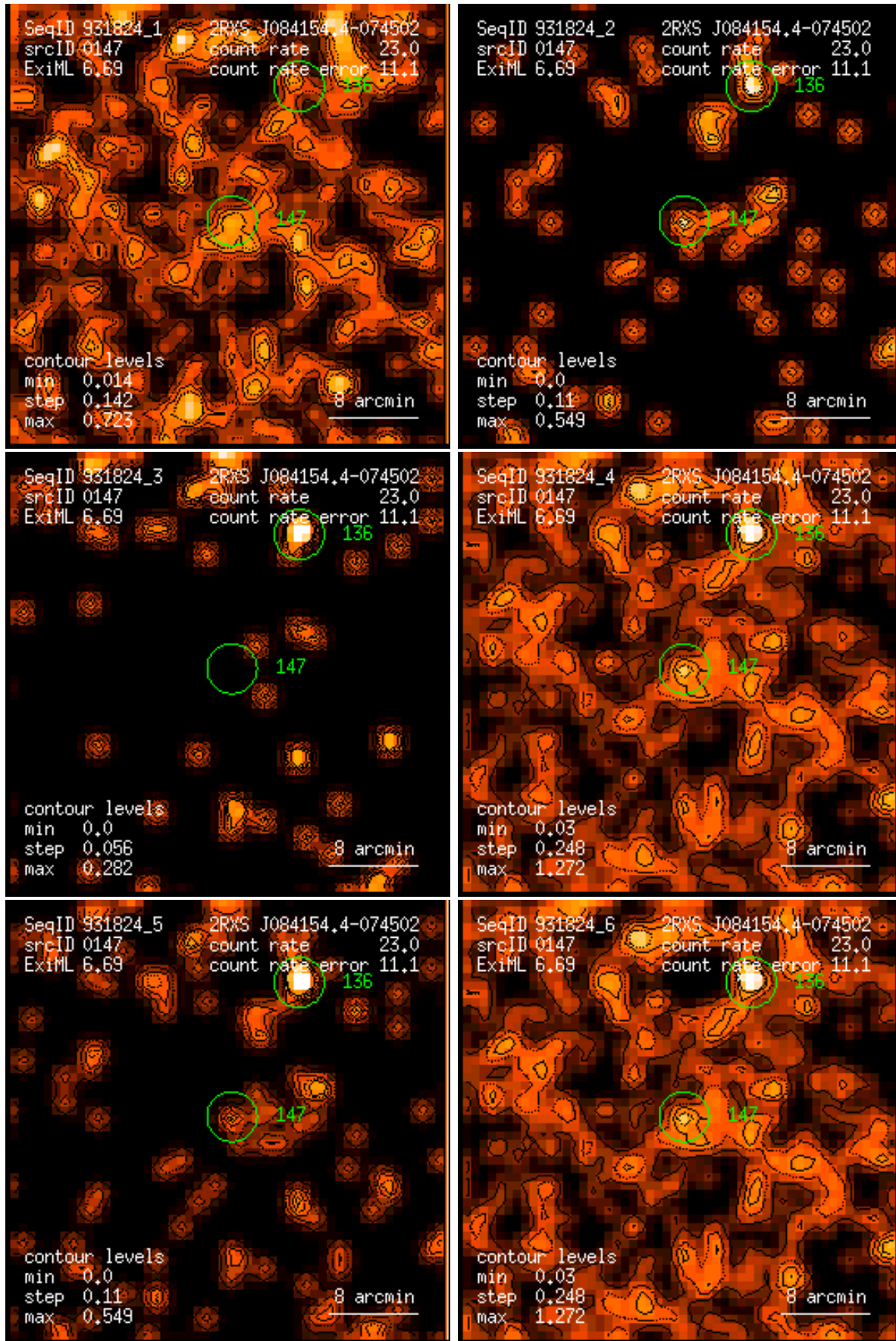
Figure 147: RASS 931824: detection 0147: band rate images, Gaussian filter: (1) PSPC channels 11 – 41, (2) 52 – 90, (3) 91 – 201, (4) 11 – 235, (5) 52 – 201, (6) 11 – 201. Broad band rates in counts/ks. Band rate contour levels in counts/ks/arcmin 2 .
