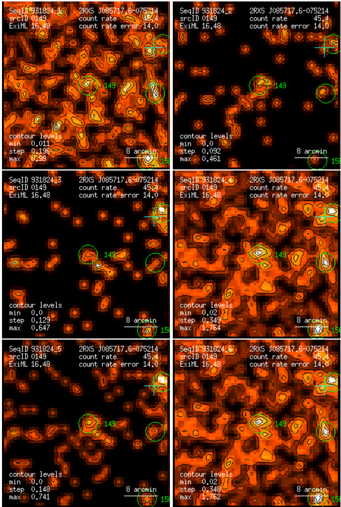
Figure 149: RASS 931824: detection 0149: band rate images, Gaussian filter: (1) PSPC channels 11 – 41, (2) 52 – 90, (3) 91 – 201, (4) 11 – 235, (5) 52 – 201, (6) 11 – 201. Broad band rates in counts/ks. Band rate contour levels in counts/ks/arcmin 2 .
