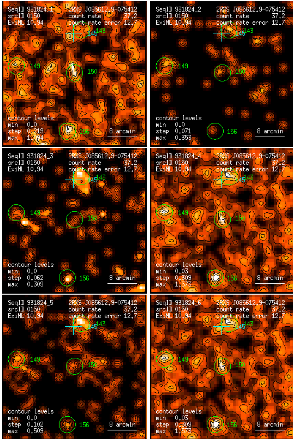
Figure 150: RASS 931824: detection 0150: band rate images, Gaussian filter: (1) PSPC channels 11 – 41, (2) 52 – 90, (3) 91 – 201, (4) 11 – 235, (5) 52 – 201, (6) 11 – 201. Broad band rates in counts/ks. Band rate contour levels in counts/ks/arcmin 2 .
