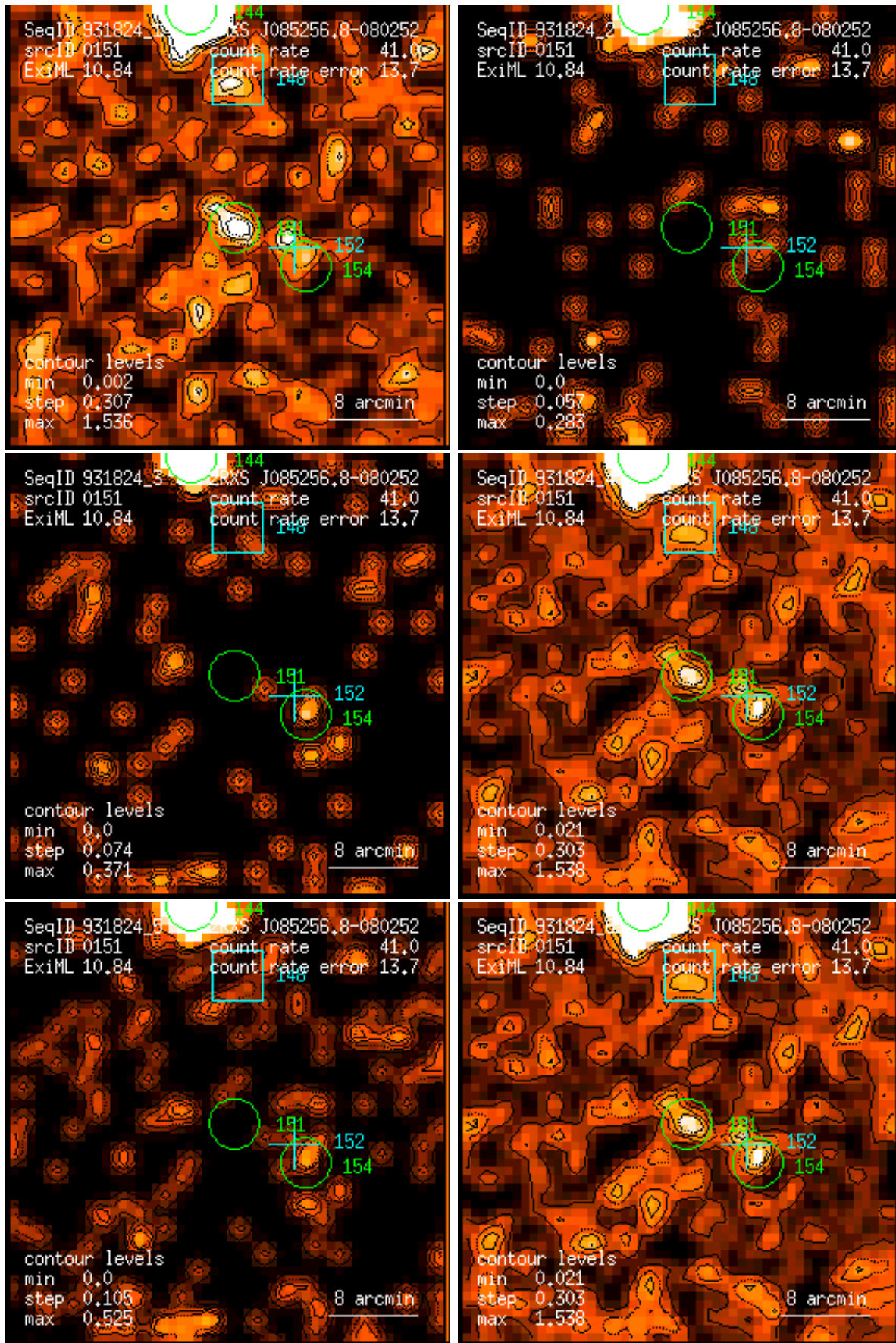
Figure 151: RASS 931824: detection 0151: band rate images, Gaussian filter: (1) PSPPC channels 11 – 41, (2) 52 – 90, (3) 91 – 201, (4) 11 – 235, (5) 52 – 201, (6) 11 – 201. Broad band rates in counts/ks. Band rate contour levels in counts/ks/arcmin 2 .
